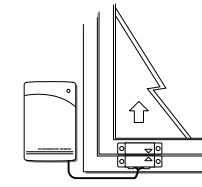
Sliding window
