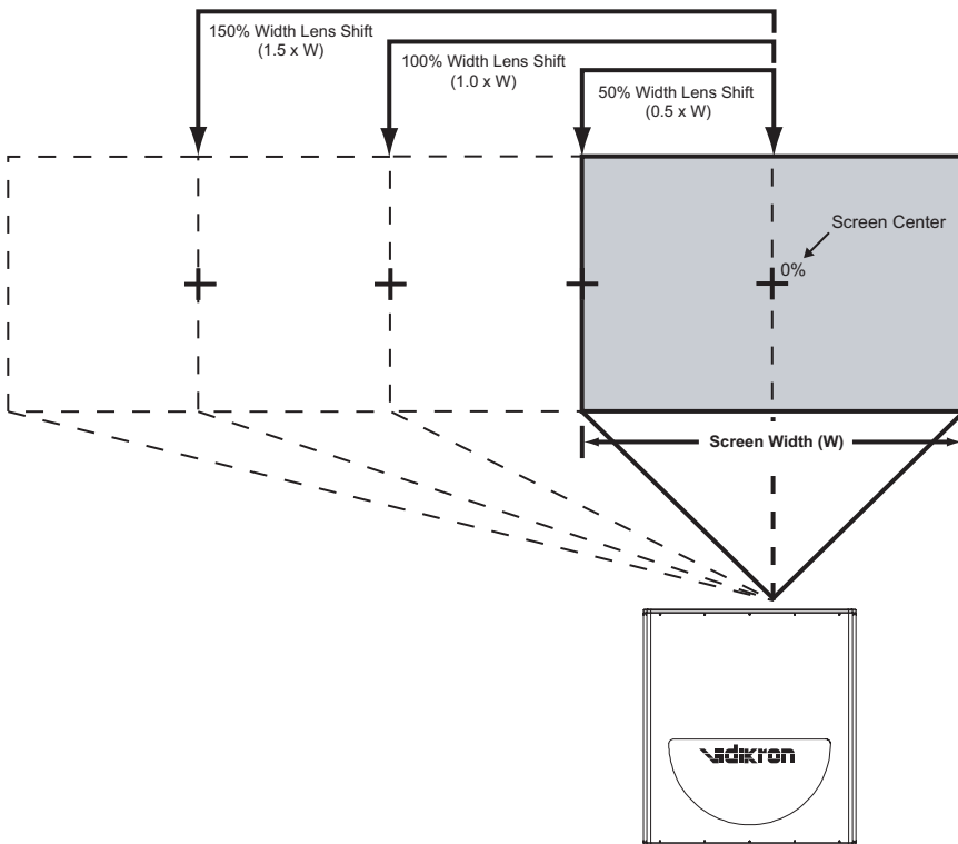
Figure 3-5. Horizontal Lens Shift
