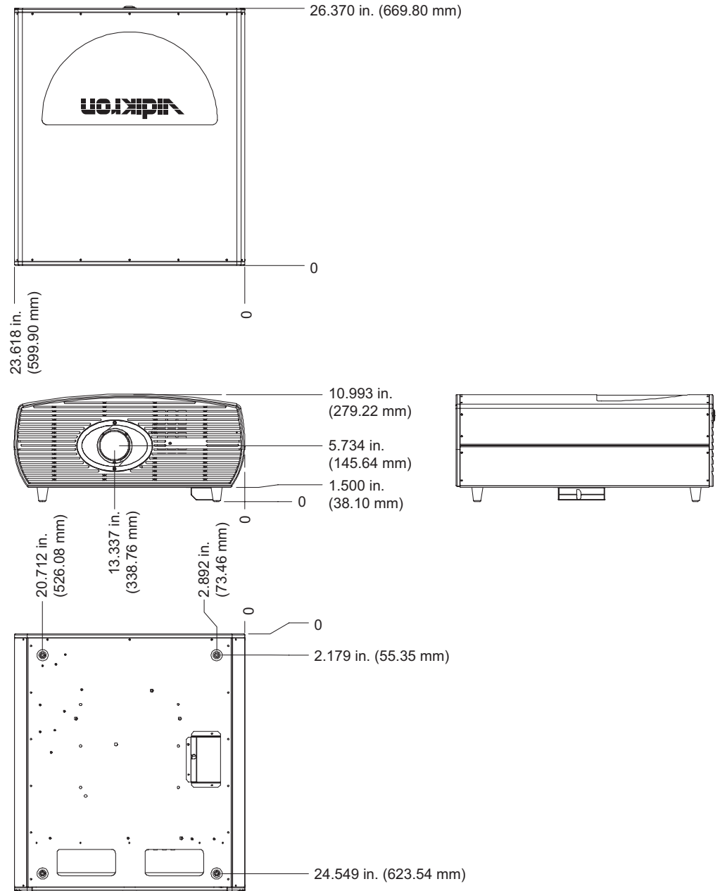
Figure 7-1. Vision 90 Dimensions
