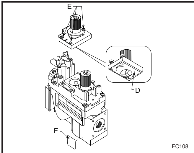
Fig. 31 Replace regulator.
