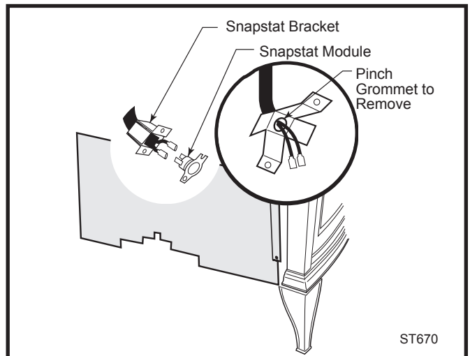
Fig. 9 Remove the snapstat and grommet from the bracket
