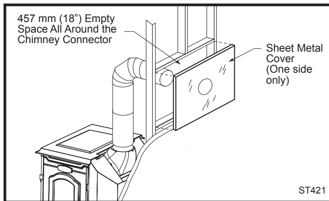
Fig. 9 Hollow wall pass-through.
