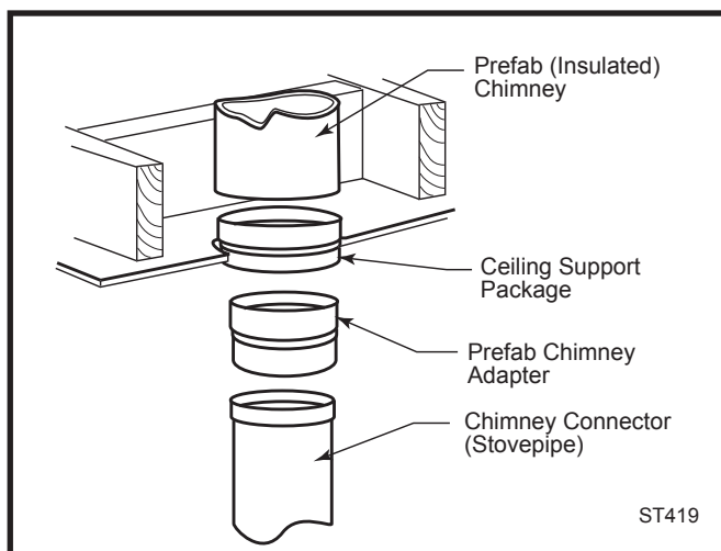
Fig. 5 Joining the chimney connector to a prefabricated chimney.
