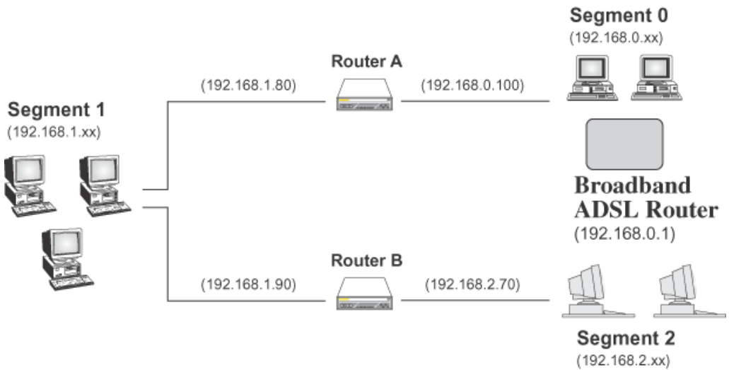
Figure 45: Routing Example
