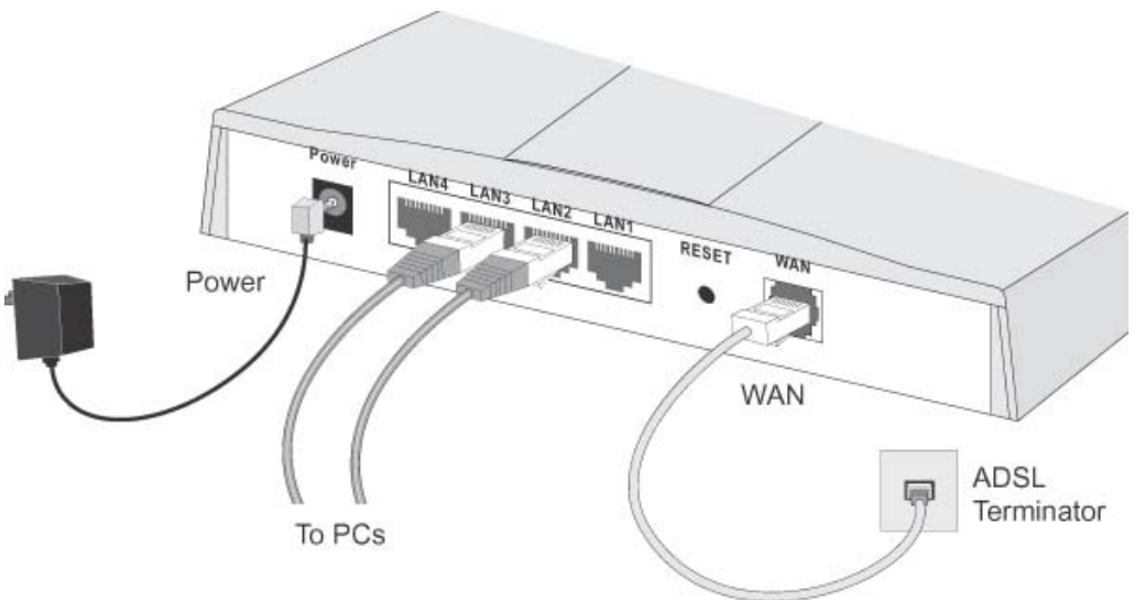
Figure 4: Installation Diagram
