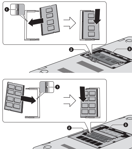
Figure 4-7 Seating the memory module
