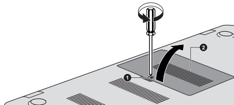
Figure 4-6 Removing the memory module cover
