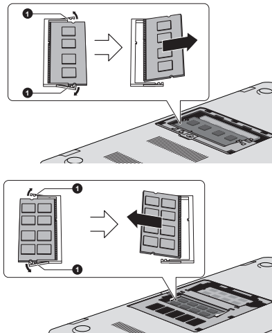
Figure 4-9 Removing the memory module
