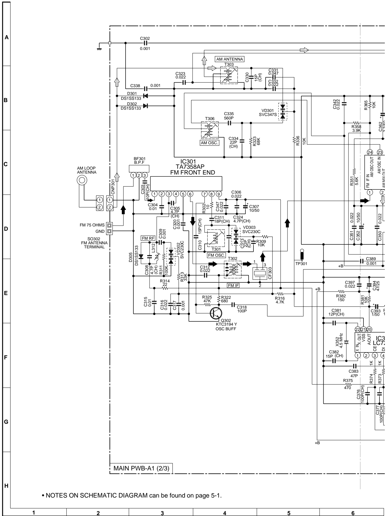
Figure 6-10 SCHEMATIC DIAGRAM (3/10)
