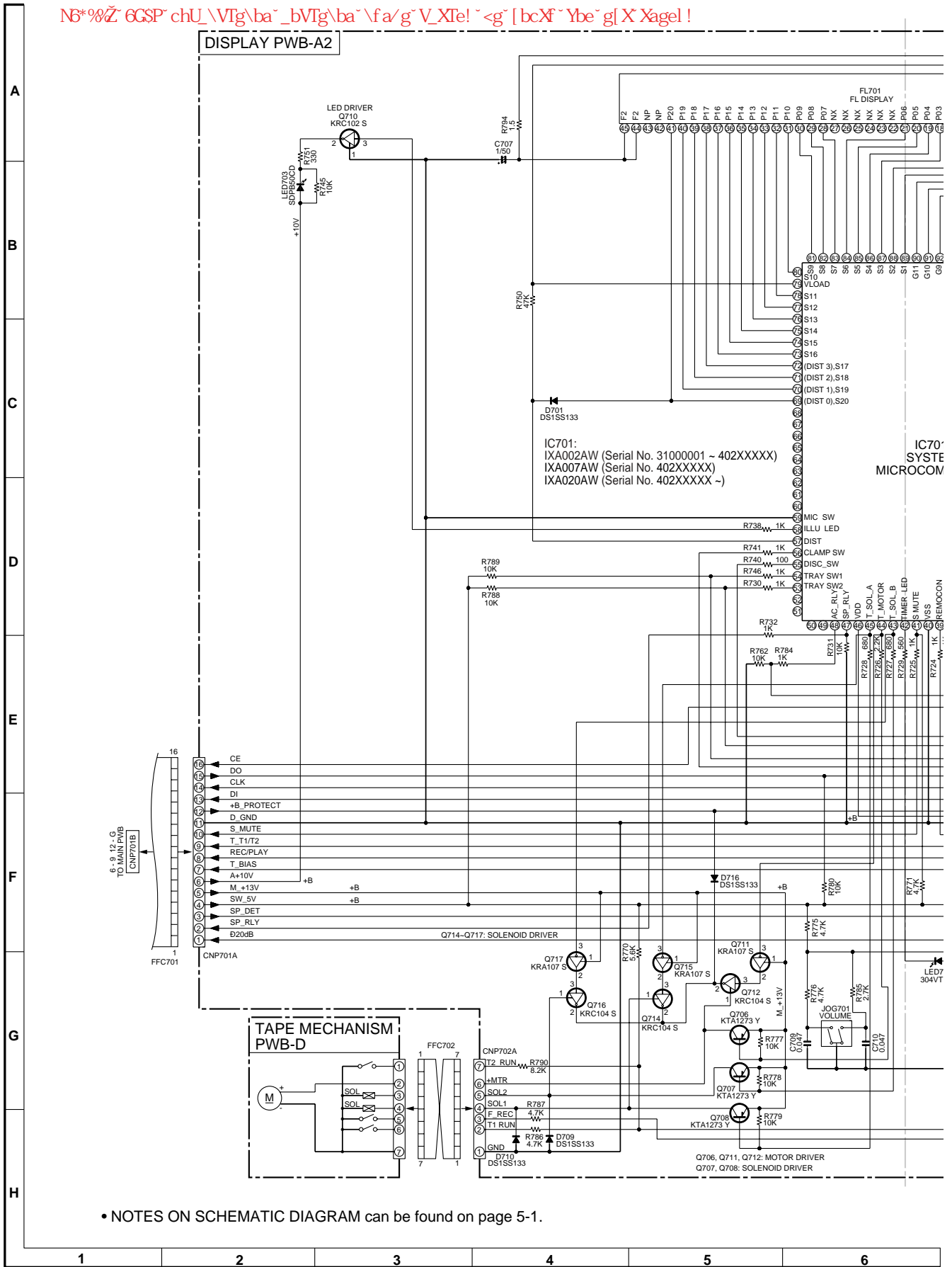
Figure 6-14 SCHEMATIC DIAGRAM (7/10)
