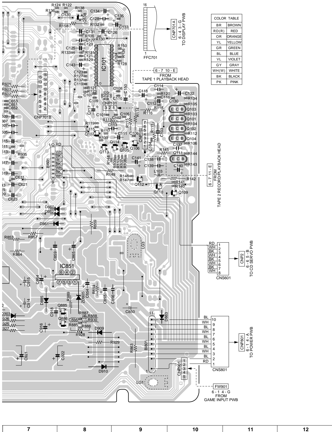
Figure 6-3 WIRING SIDE OF P.W.BOARD (3/7)
