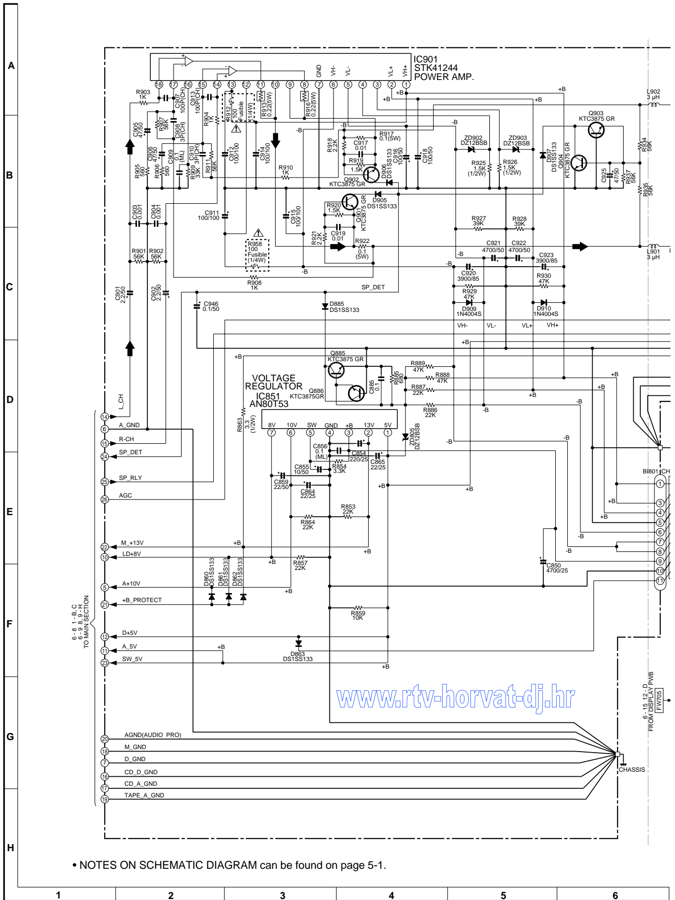
Figure 6-12 SCHEMATIC DIAGRAM (5/10)
