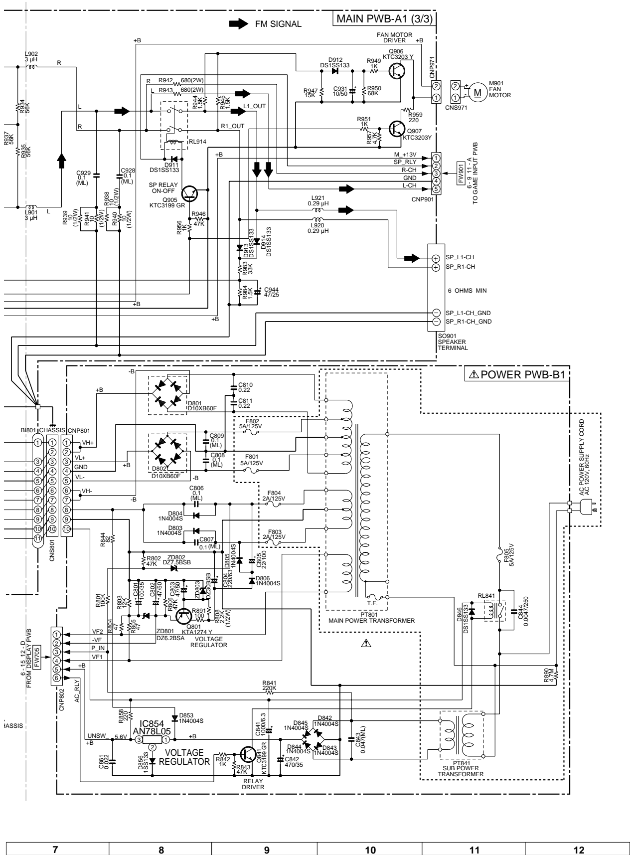
Figure 6-13 SCHEMATIC DIAGRAM (6/10)
