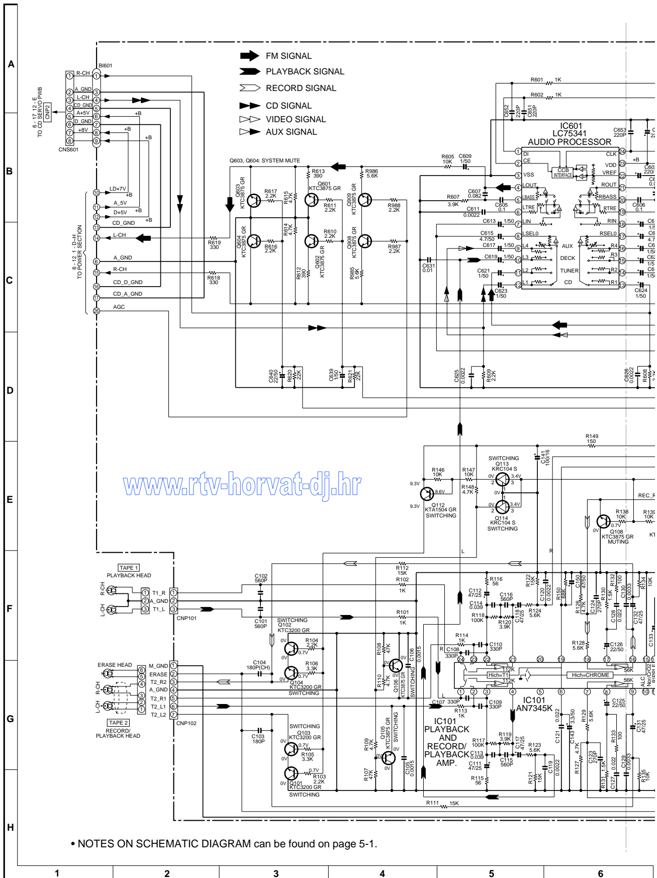
Figure 6-8 SCHEMATIC DIAGRAM (1/10)
