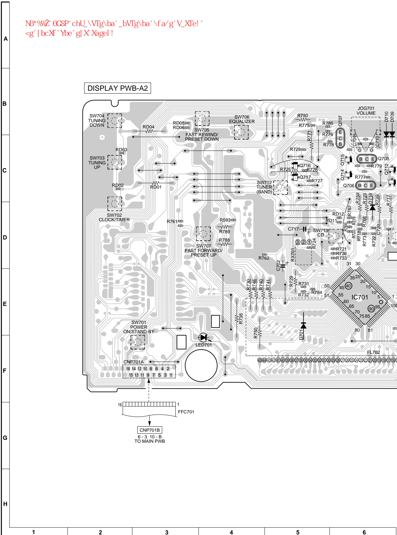
Figure 6-4 WIRING SIDE OF P.W.BOARD (4/7)
