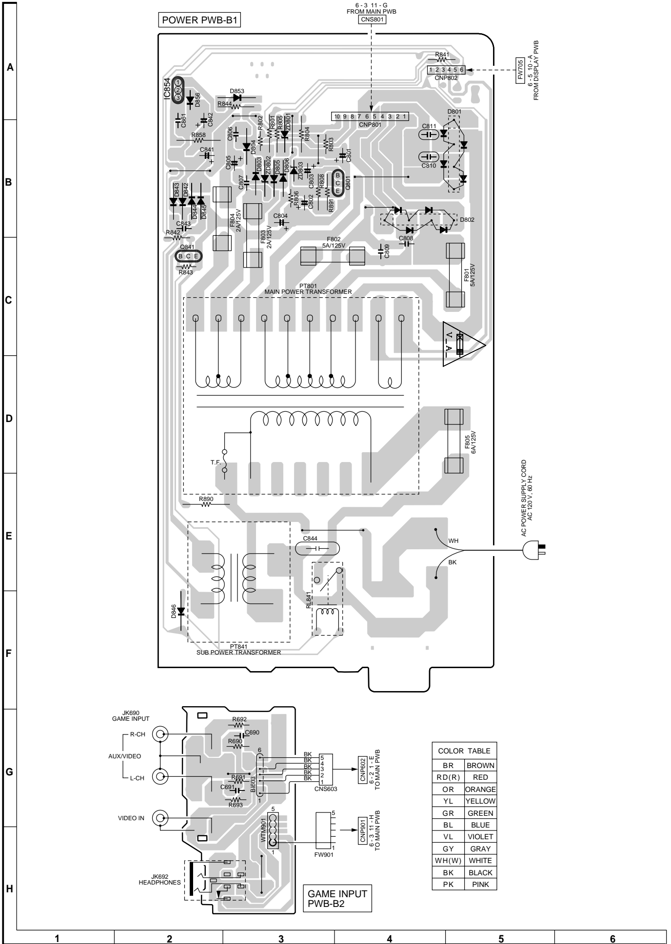
Figure 3 WIRING SIDE OF PWB (1/1)
