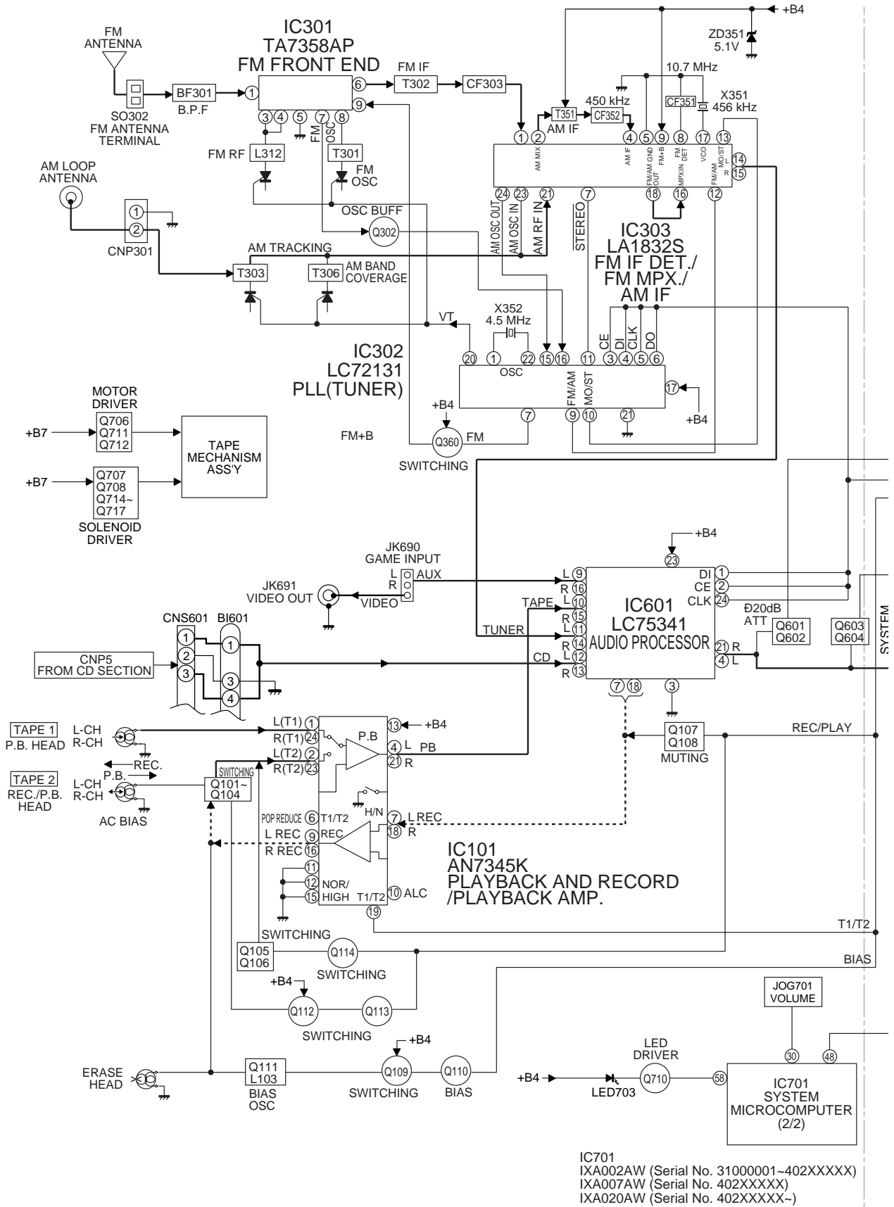
Figure 4-2 BLOCK DIAGRAM (2/3)
