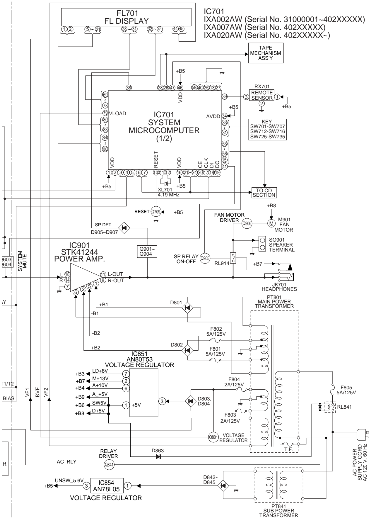
Figure 4-3 BLOCK DIAGRAM (3/3)
