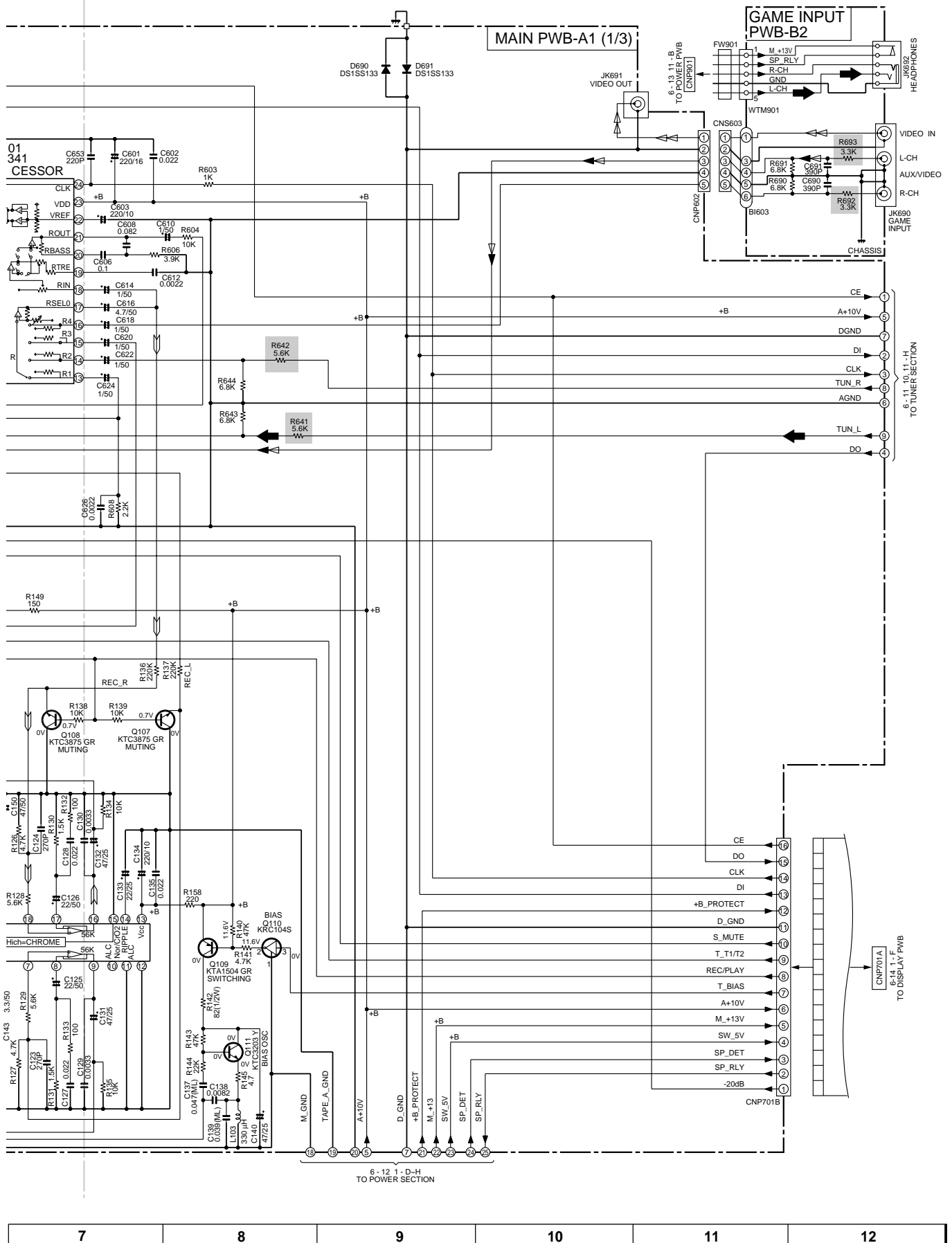
Figure 5 SCHEMATIC DIAGRAM (2/3)
