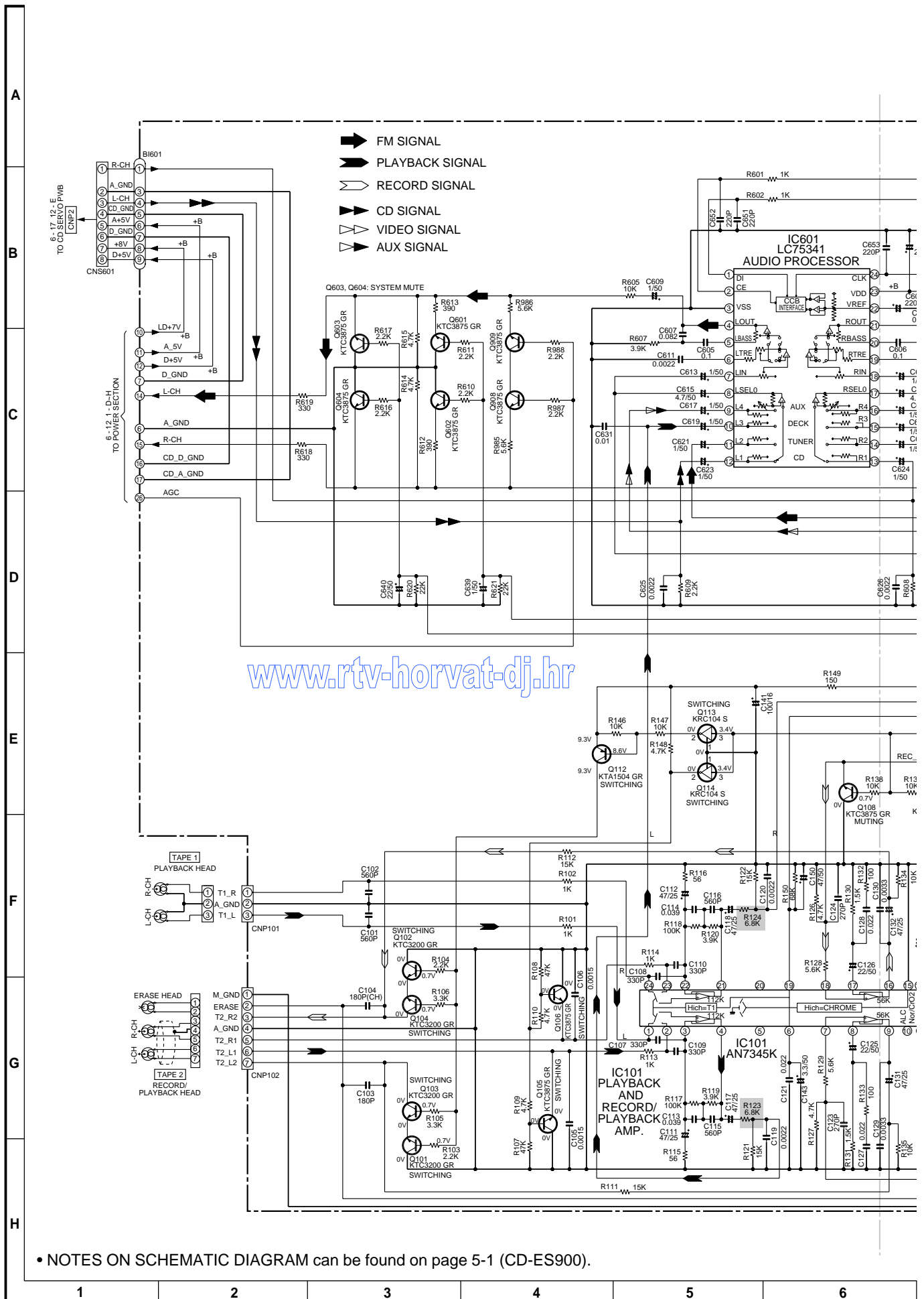
Figure 4 SCHEMATIC DIAGRAM (1/3)
