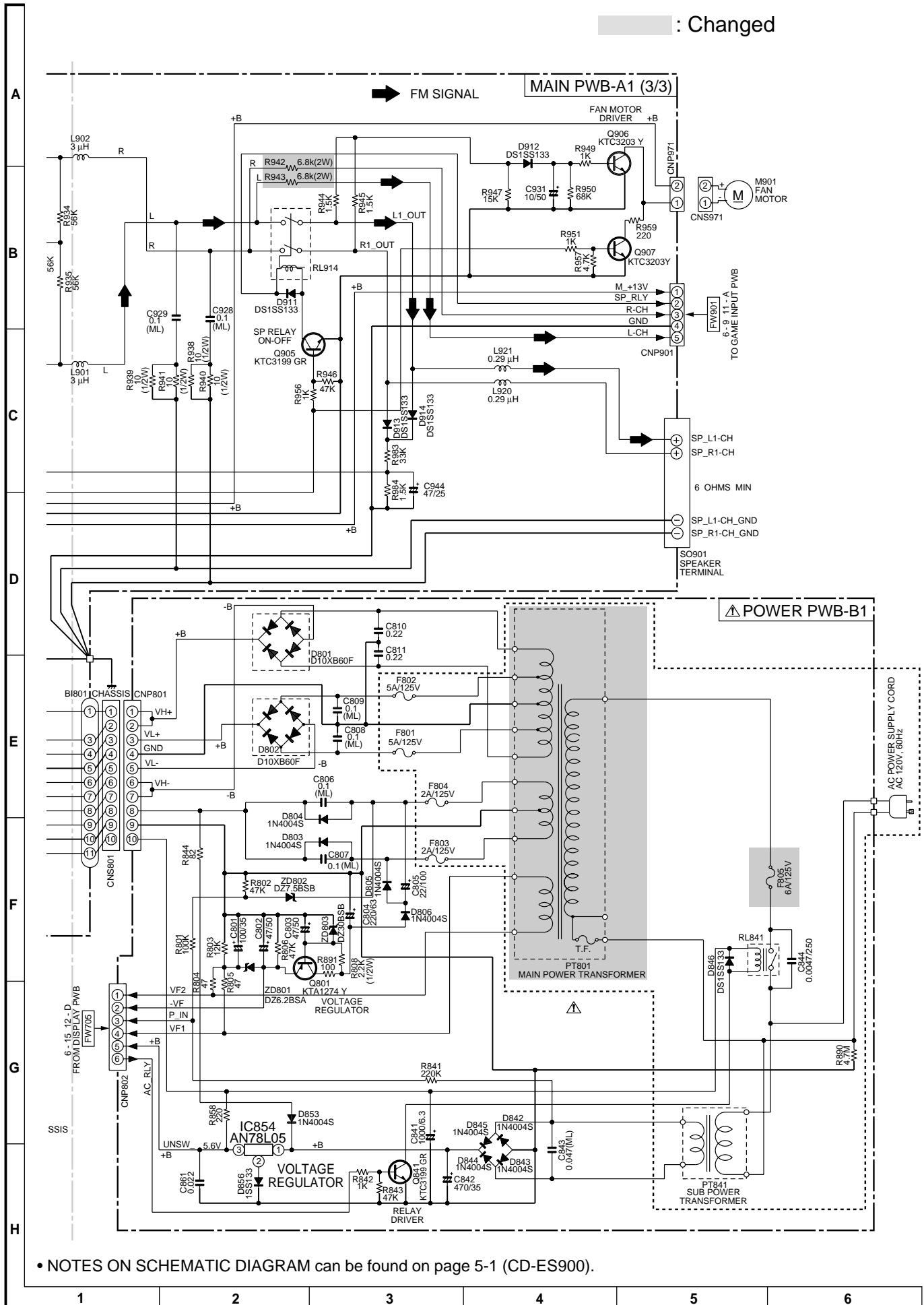
Figure 6 SCHEMATIC DIAGRAM (3/3)
