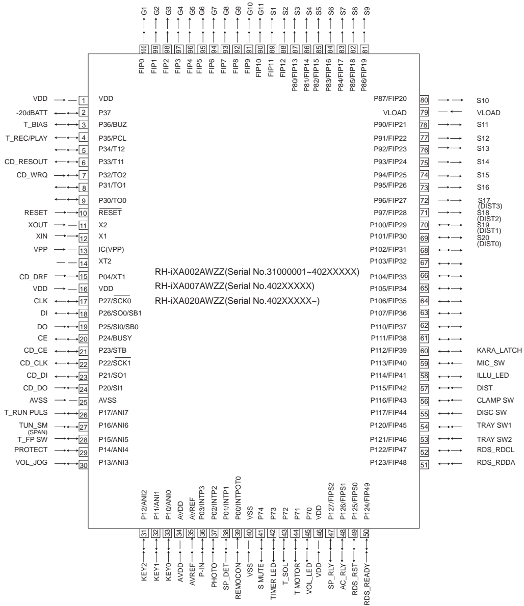
Figure 8-8 BLOCK DIAGRAM OF IC
