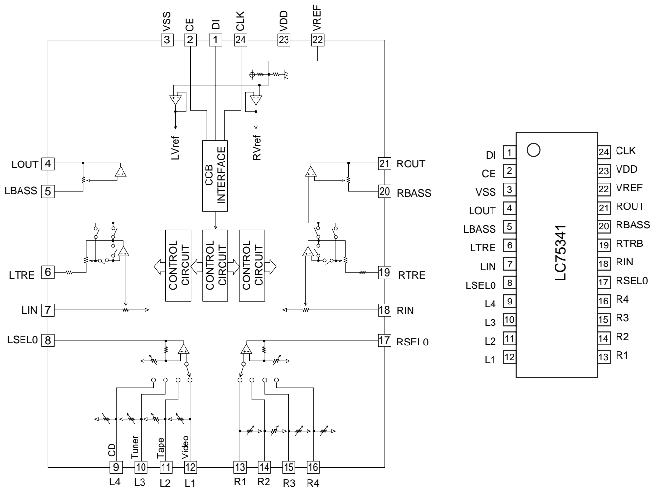
Figure 8-5 BLOCK DIAGRAM OF IC
