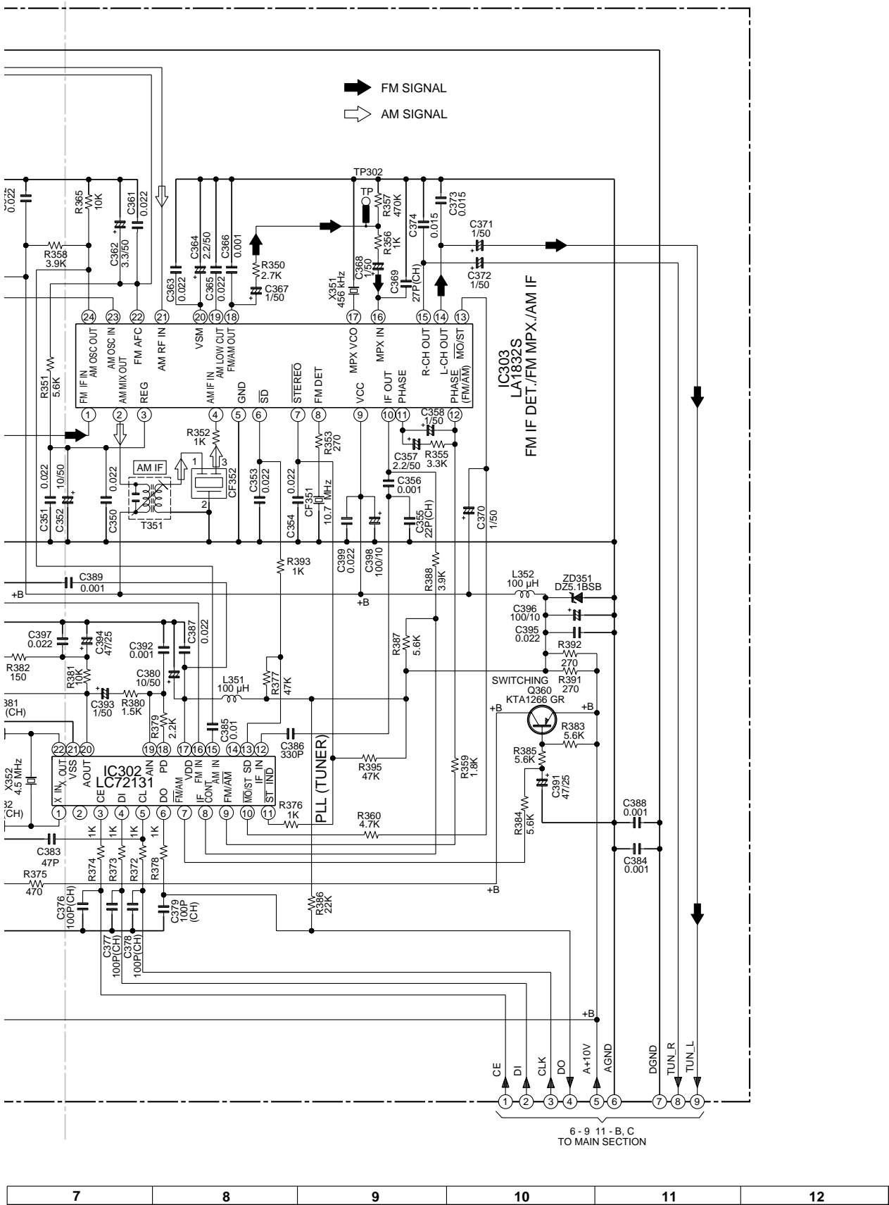
Figure 6-11 SCHEMATIC DIAGRAM (4/10)
