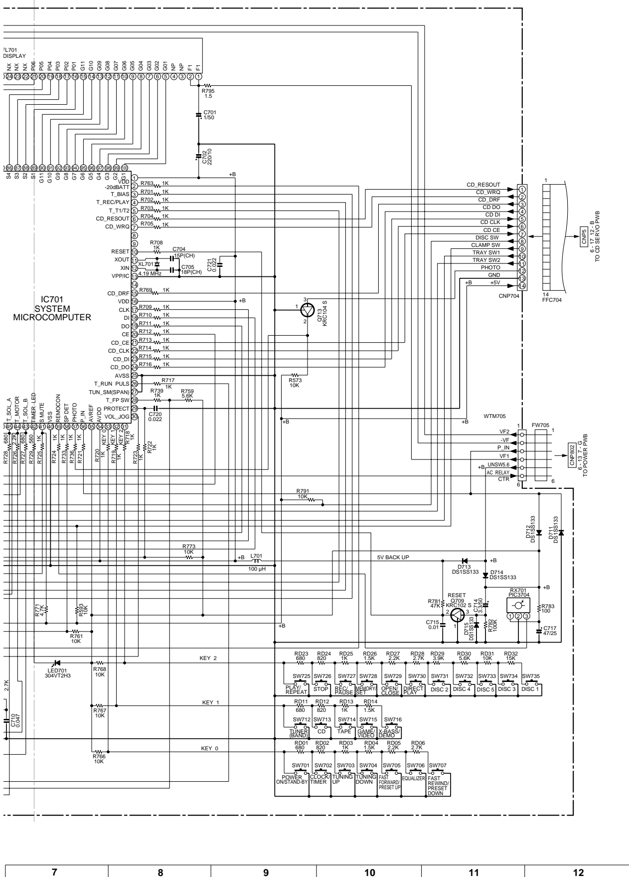
Figure 6-15 SCHEMATIC DIAGRAM (8/10)
