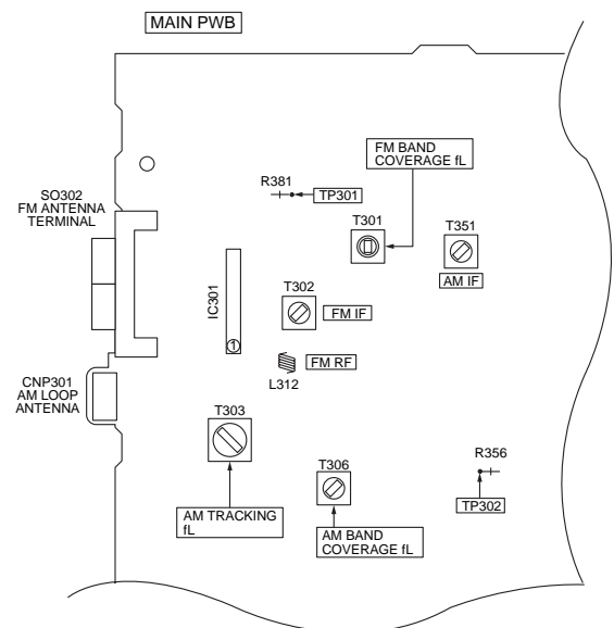
Figure 2 ADJUSTMENT POINTS
