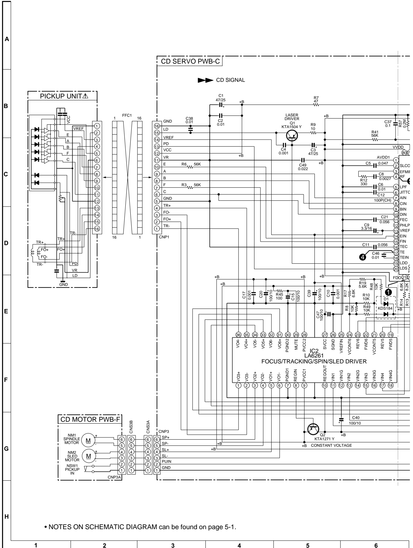
Figure 6-16 SCHEMATIC DIAGRAM (9/10)
