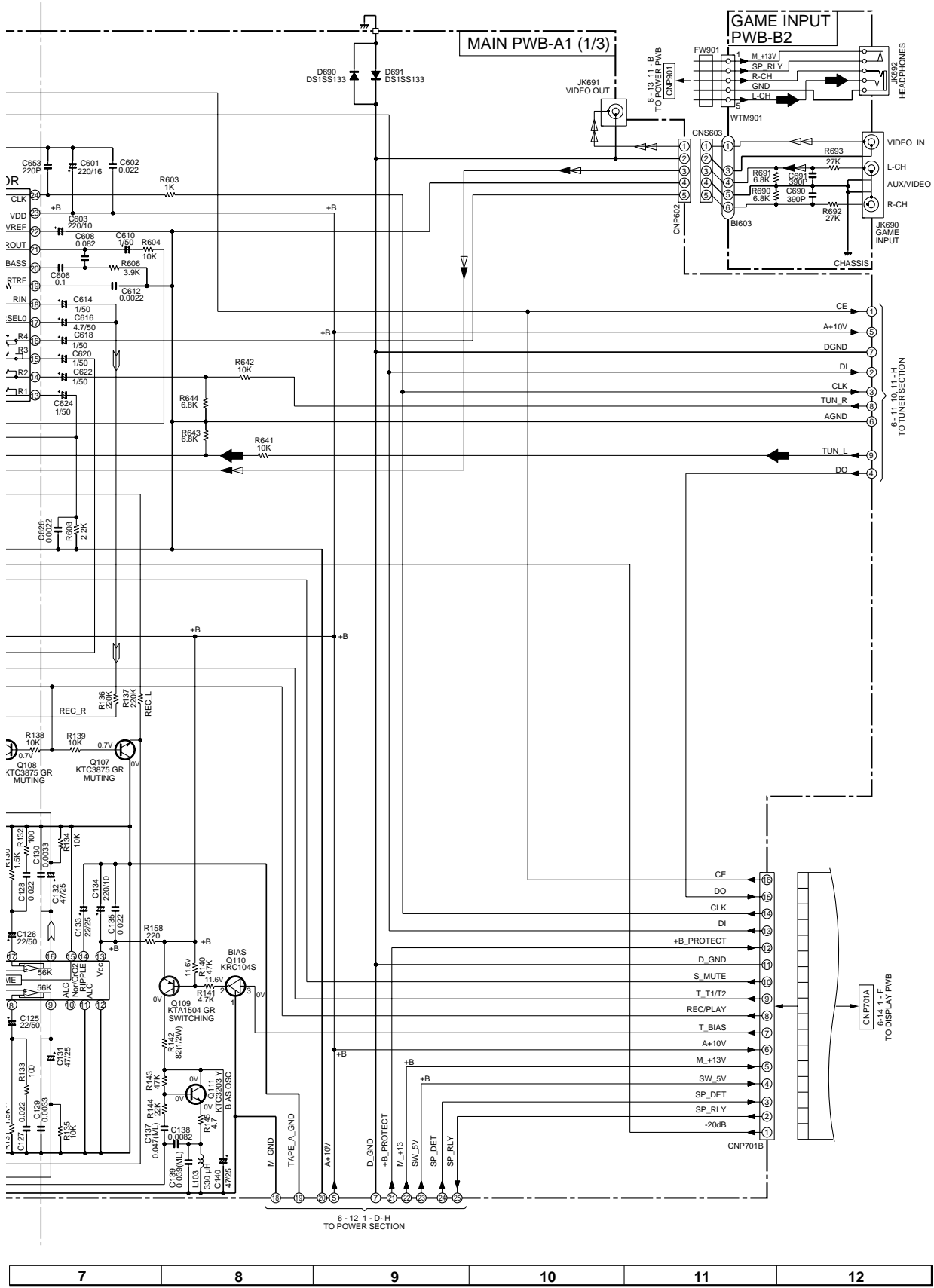
Figure 6-9 SCHEMATIC DIAGRAM (2/10)
