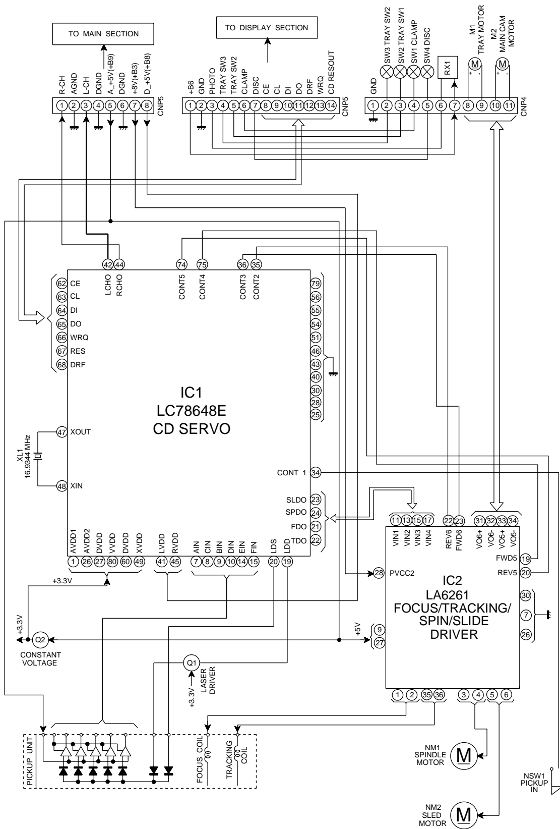
Figure 4-1 BLOCK DIAGRAM (1/3)
