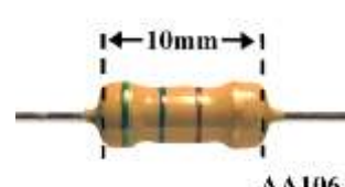
560E 5% 0.5 Watt Carbon Film Resistor AA106 R0475 R 0.71
