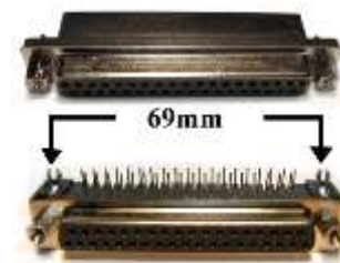
25 Pin D-Sub con. Socket right angle PCB
