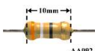
39E 5% 0.5 Watt Carbon Film Resistor AA092 R1521 R 0.48
