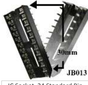
IC Socket 24 Standard Pin DIP 0.3 inch
