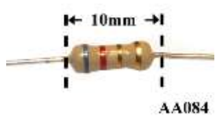
8.2E 5% 0.5 Watt Carbon Film Resistor AA084 G0370 R 0.55
