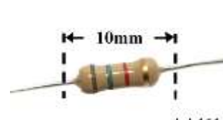
1.5K 5% 0.5 Watt Carbon Film Resistor AA111 R0590 R 0.48
