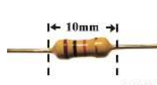
1K 5% 0.5 Watt Carbon Film Resistor AA109 R0105 R 0.6
