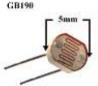
LDR Photoresistor 4-7kOhm 5mm Diameter
