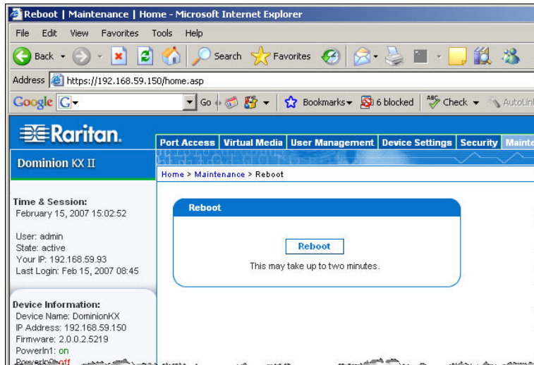
Figure 86: Reboot
