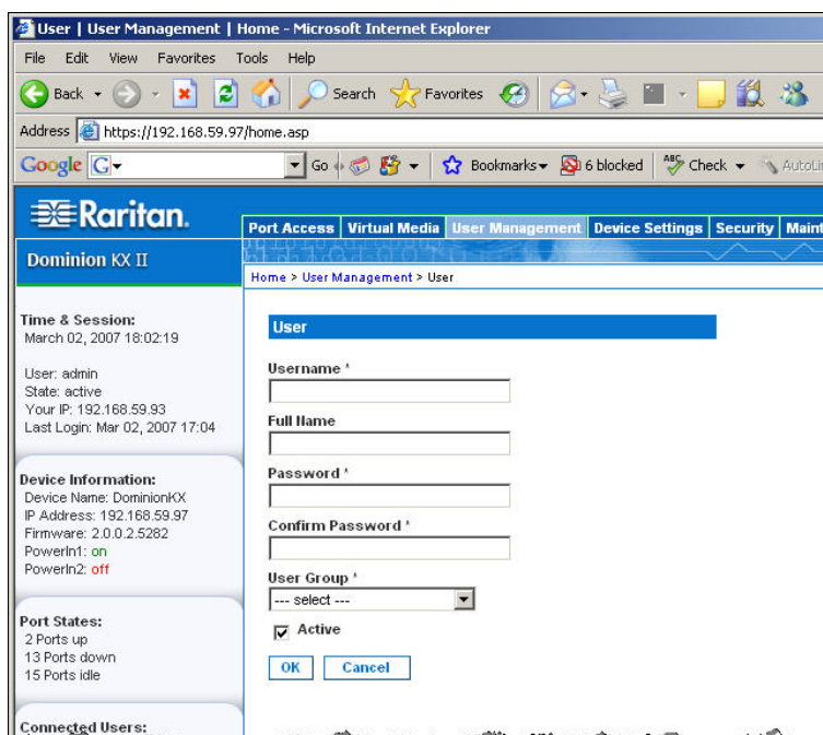
Figure 45: User Page
