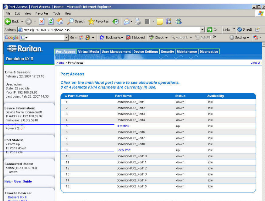
Figure 23: Port Access
