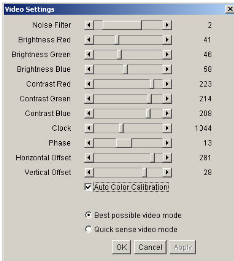
Figure 35: Video Settings
