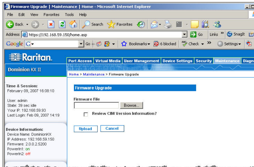
Figure 82: Firmware Upgrade
