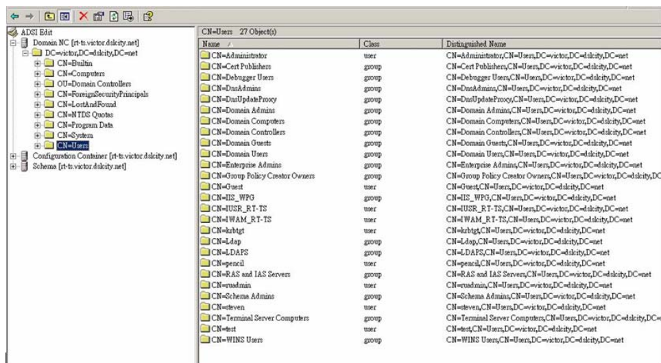
Figure 110: ADSI Edit
