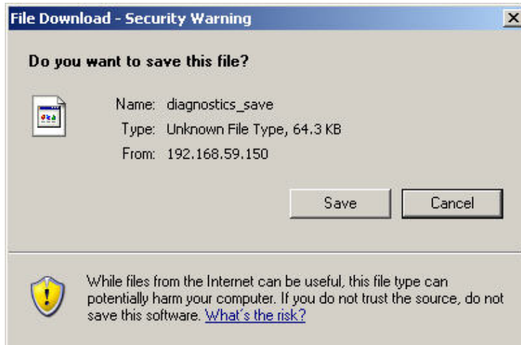
Figure 97: File Download
