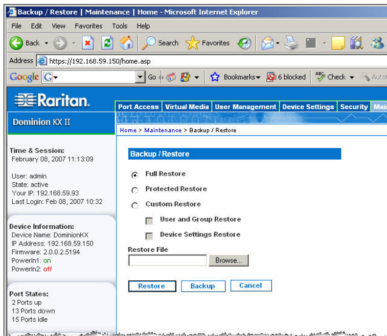
Figure 80: Backup/Restore
