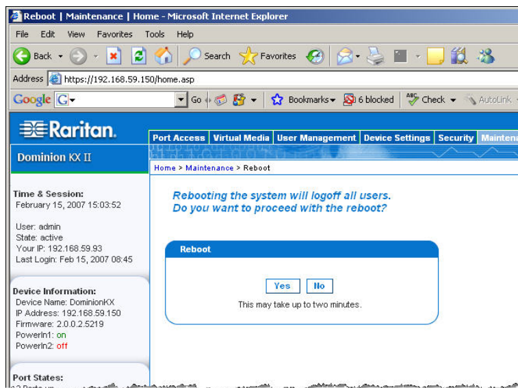
Figure 87: Reboot Confirmation
