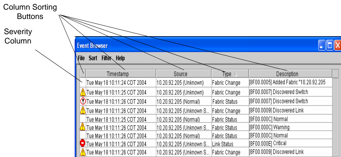
Figure 3-11. Events Browser
