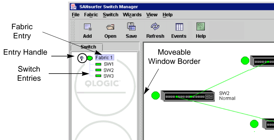
Figure 2-9. Fabric Tree
