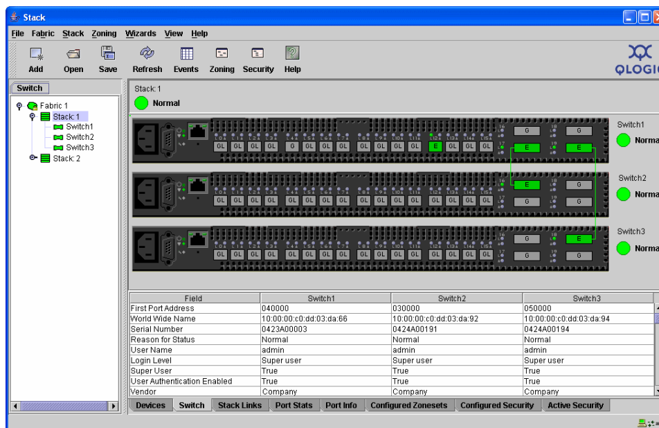
Figure 4-14. Switch Stacks
