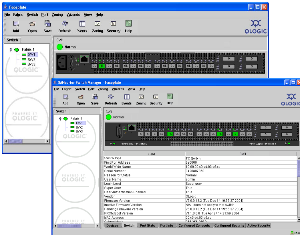
Figure 2-11. Faceplate Display
