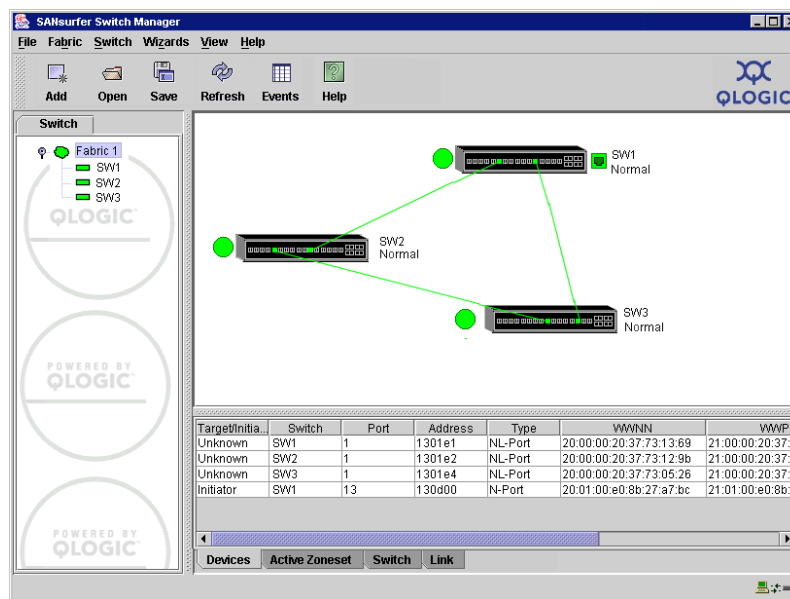
Figure 2-10. Topology Display
