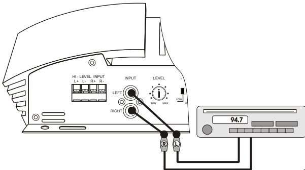
TWO CHANNEL SIGNAL CONNECTIONS
