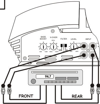
FOUR CHANNEL SIGNAL CONNECTIONS (RADIO WITH FRONT AND REAR OUTPUTS)
