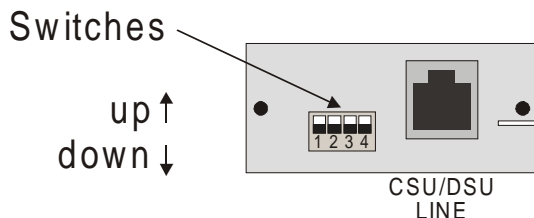
Figure 3-1 Rear View of ATL-CSU/DSU Link Module Switches
