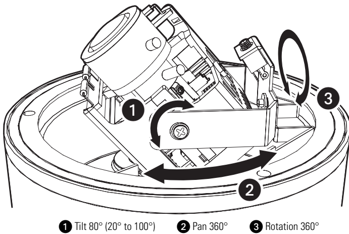
Figure 15. Positioning the Camera
