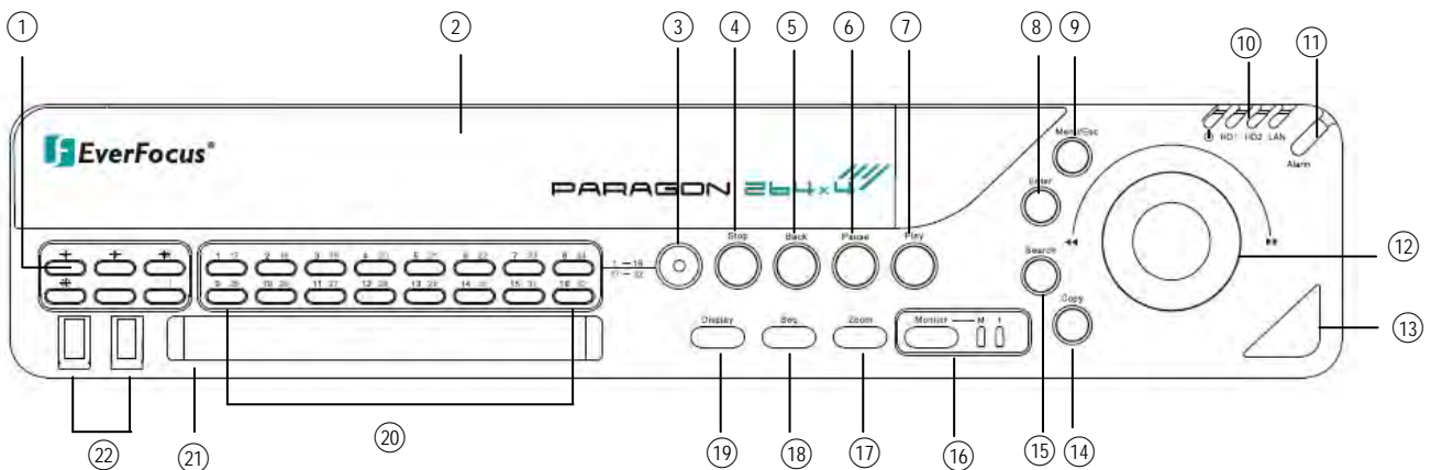
Figure 1-1 Front Panel
