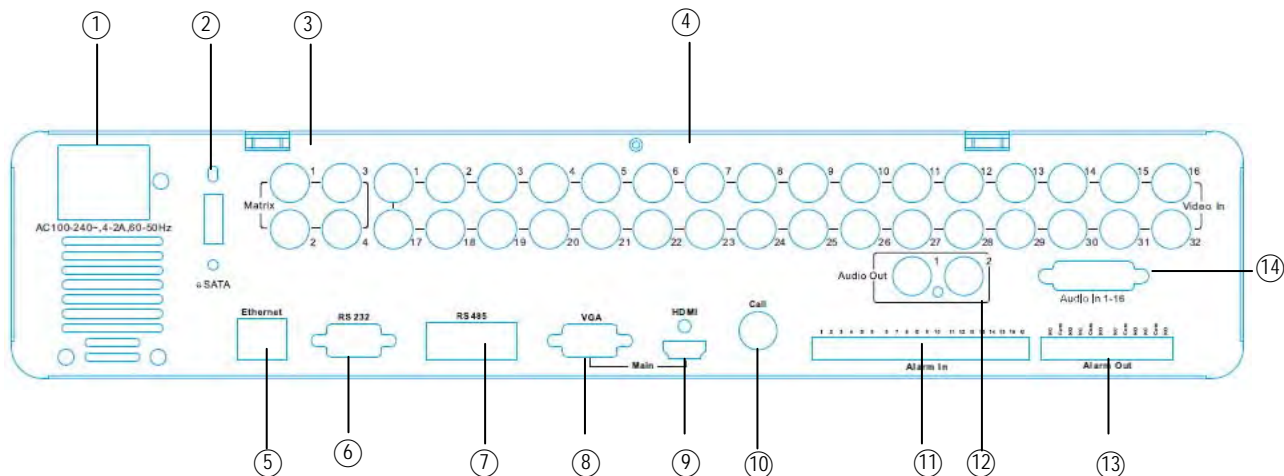
Figure 1-2 Rear Panel
