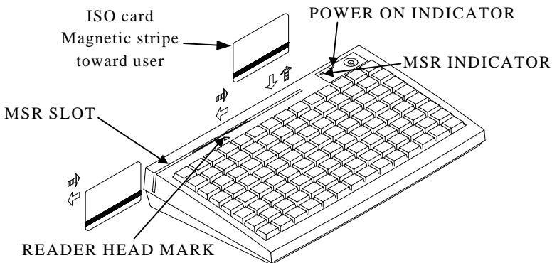
Fig. 4 - 3 Reading magnetic stripe cards of ISO standard
