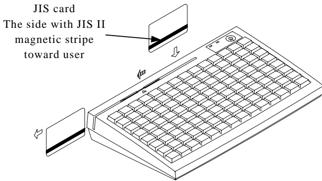
Fig. 4 - 4 Reading magnetic stripe cards of JIS standard
