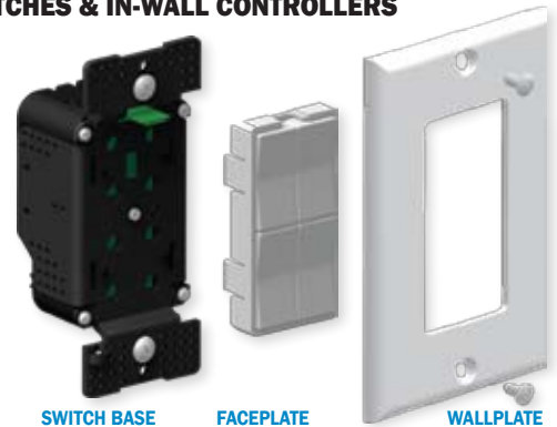
SWITCH BASE
