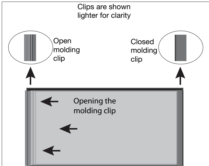
Step 1. WS-55517 and WS-65517 Diamond Shield molding clip removal
