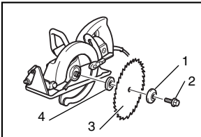
1. Outer flange 2. Hex bolt 3. Saw blade 4. Inner flange
