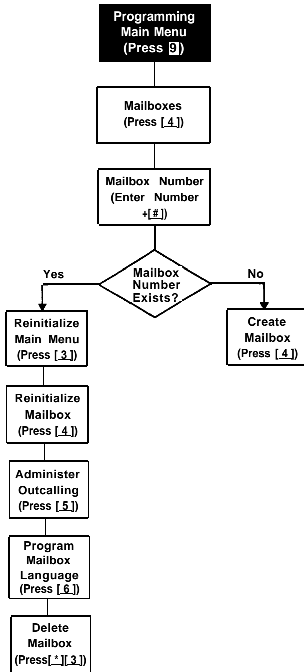
Figure 5-3. Modifying Mailboxes
