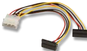
5.25" Power to 2 x 90° 15 Way SATA Power Male
