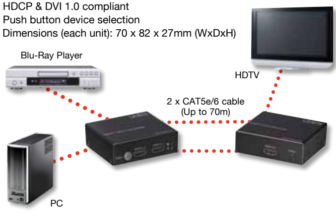
70m CAT5e 2 Port Switching HDMI Extender Part No. 38000
