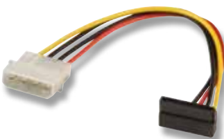
5.25" Power to 90° 15 Way SATA Power Male
