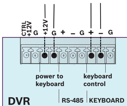
Figure 5.1: RJ11 adapter connections
