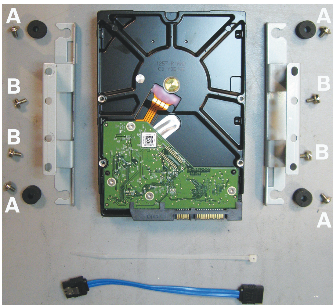
Figure 11.4: HDD install components for DIVAR AN 3000
