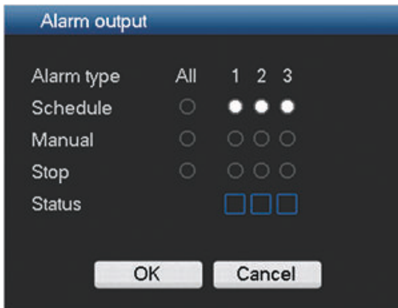
Figure 6.32: Alarm output
