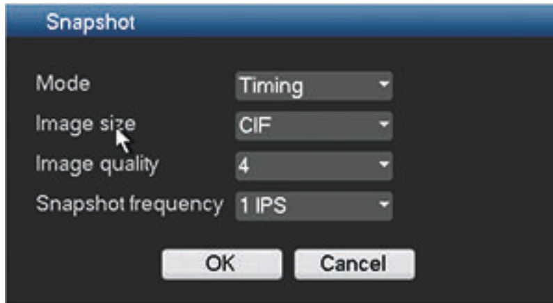
Figure 6.6: Encode snapshot
