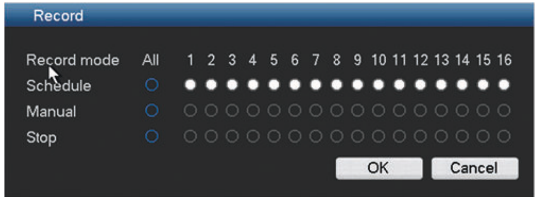
Figure 6.33: Record
