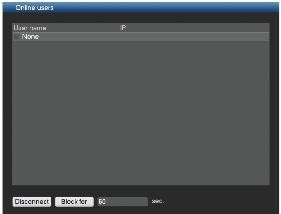
Figure 7.16: Online users
