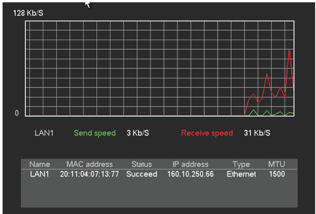
Figure 7.18: Net load
