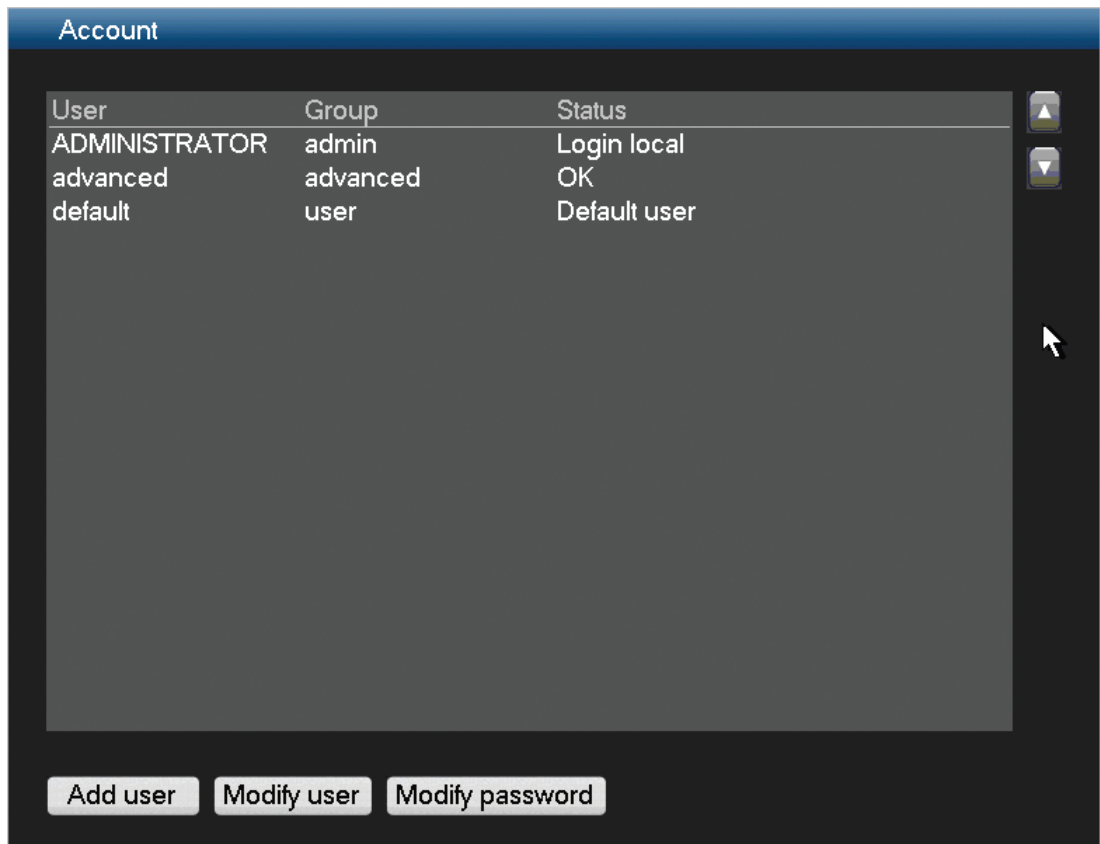
Figure 6.34: Account
