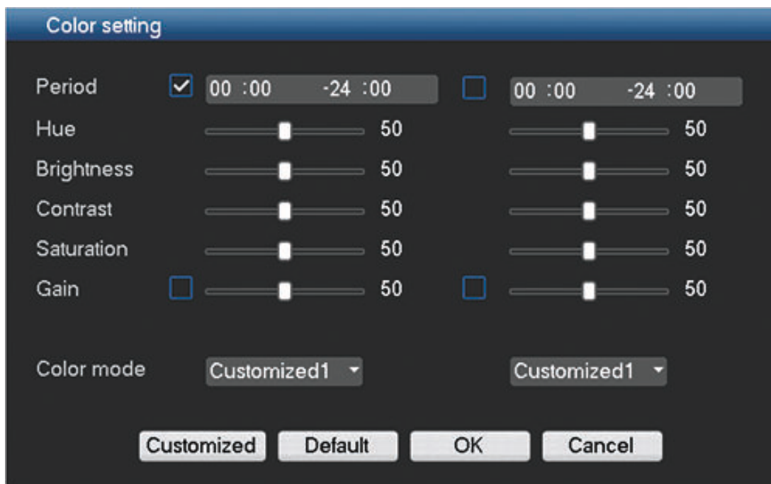
Figure 7.4: Color setting
