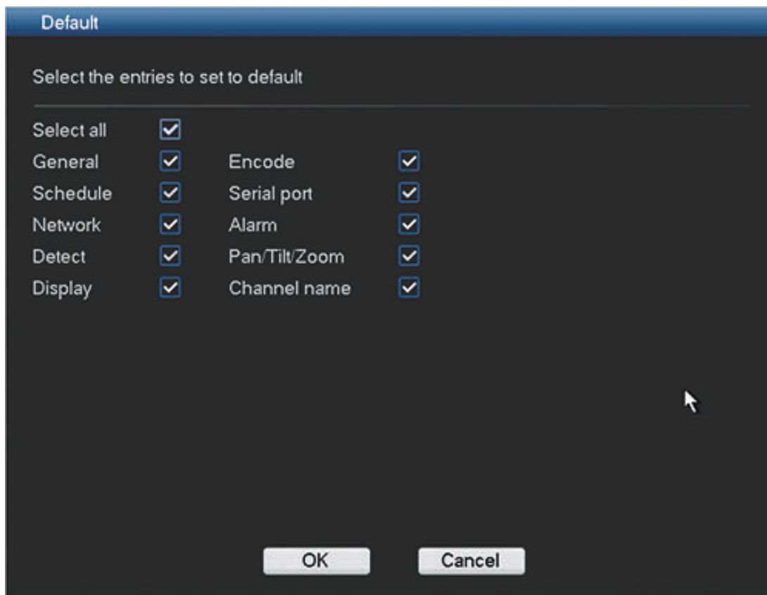
Figure 6.28: Default
