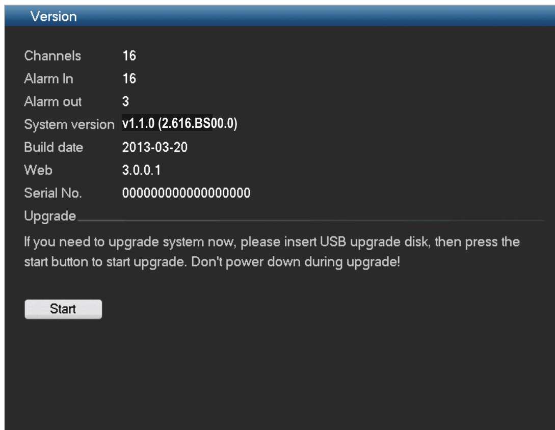
Figure 7.15: Version
