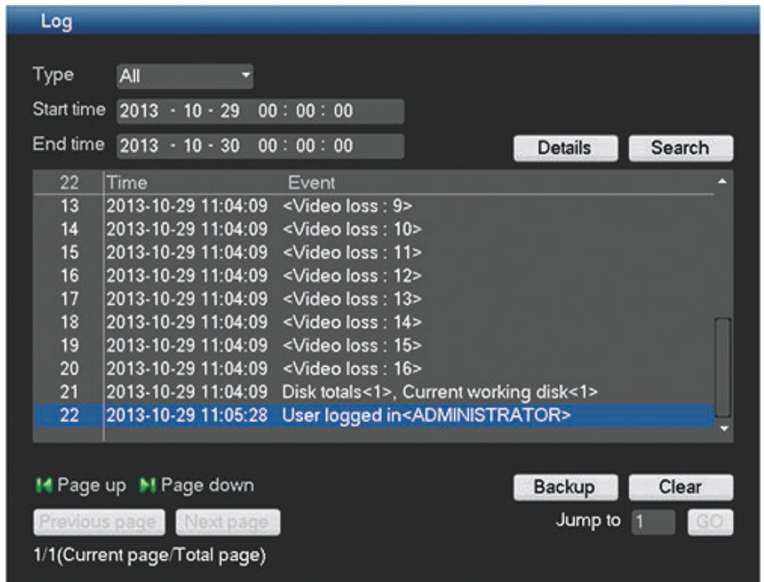
Figure 7.14: Log info
