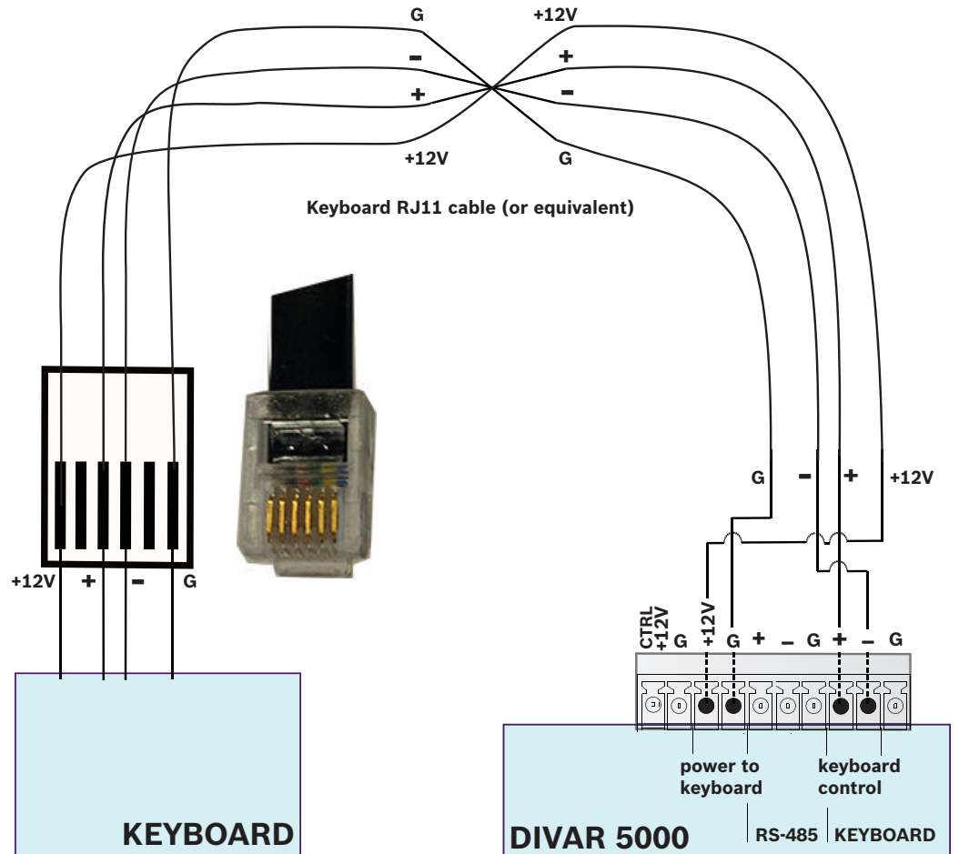
Figure 5.2: Cable connections
