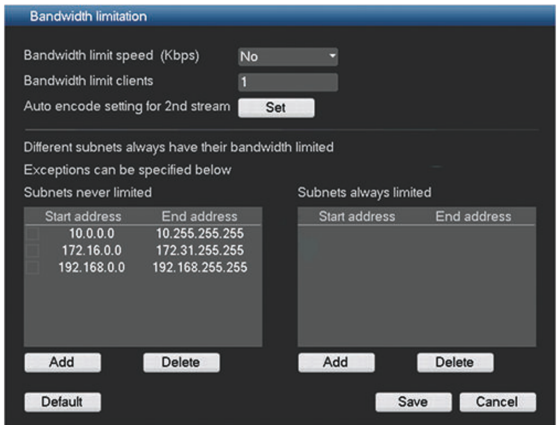
Figure 6.10: Configure bandwidth
