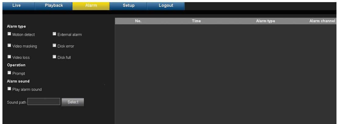
Figure 8.4: Web alarm
