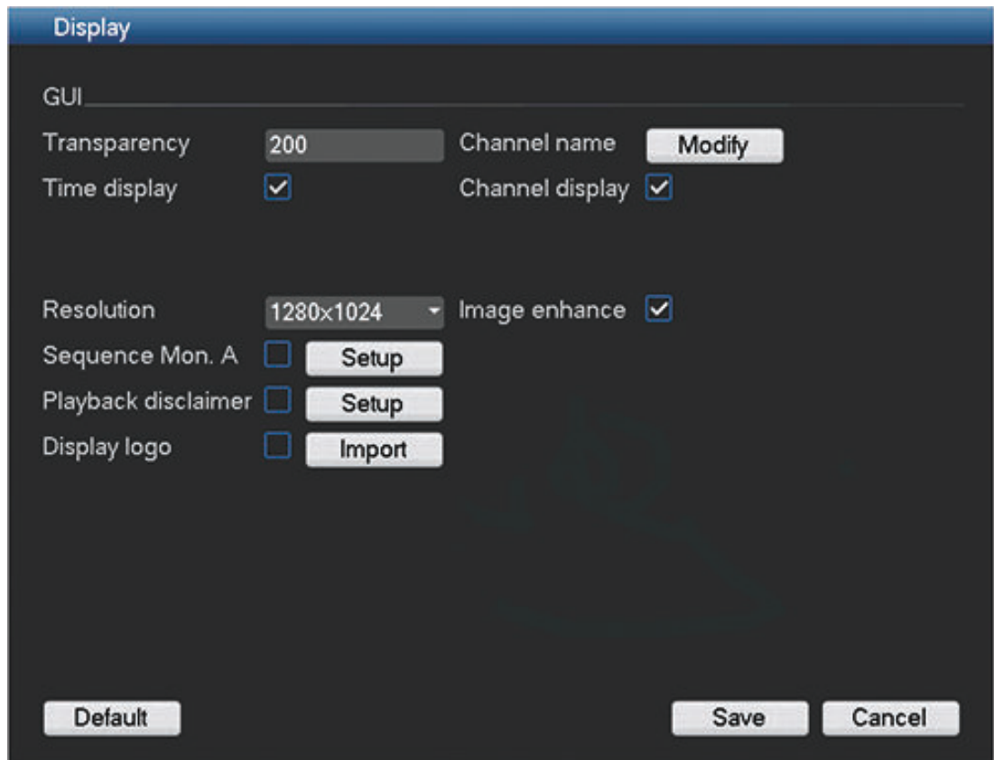
Figure 6.26: Display
