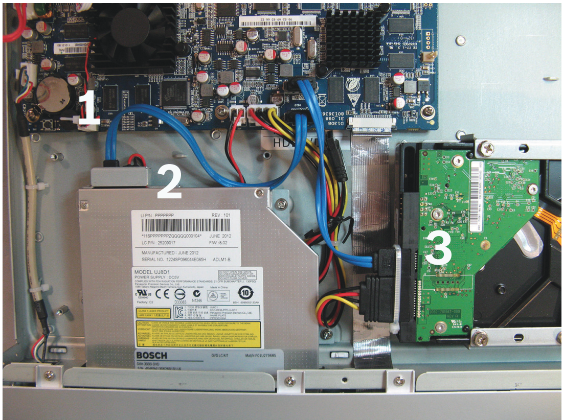
Figure 11.1: DIVAR AN 3000
