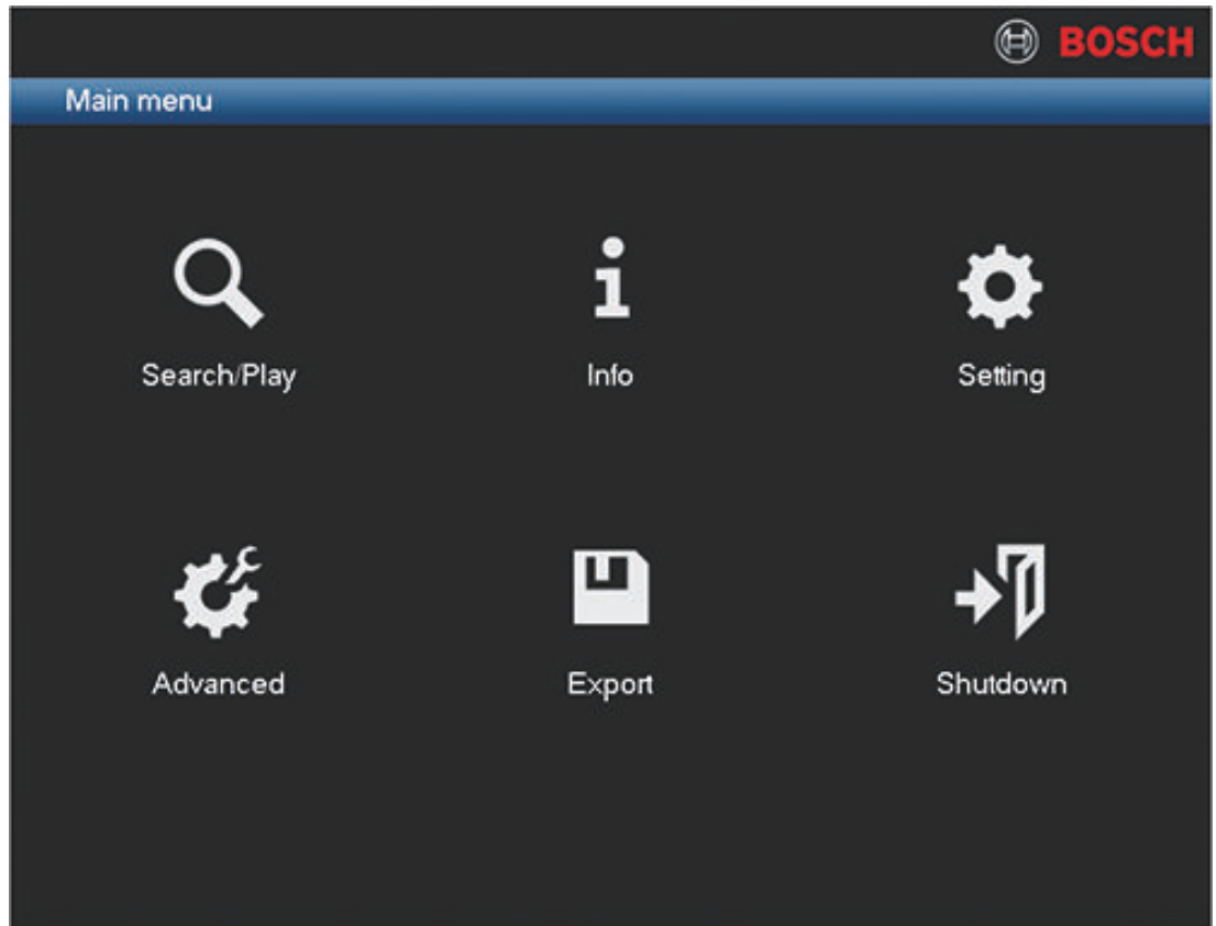
Figure 7.5: Main menu
