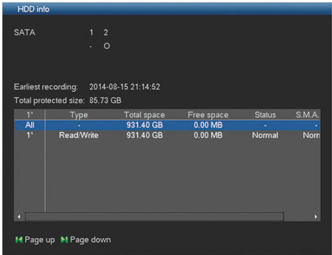
Figure 7.11: HDD info
