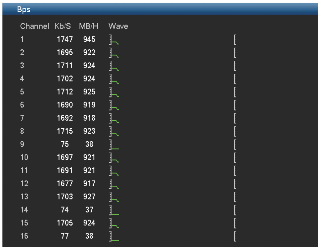
Figure 7.13: Bps
