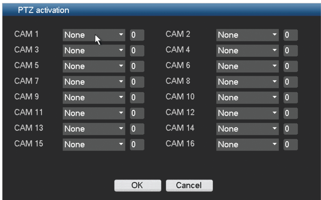
Figure 6.24: PTZ activation
