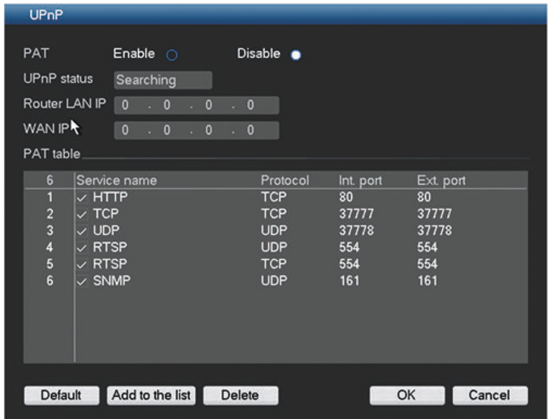
Figure 6.16: Network UPnP
