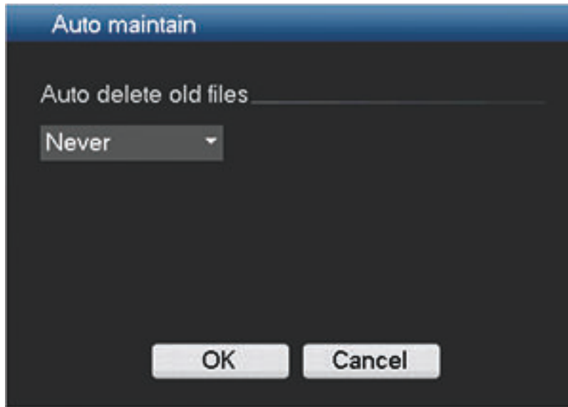
Figure 6.38: Auto maintain
