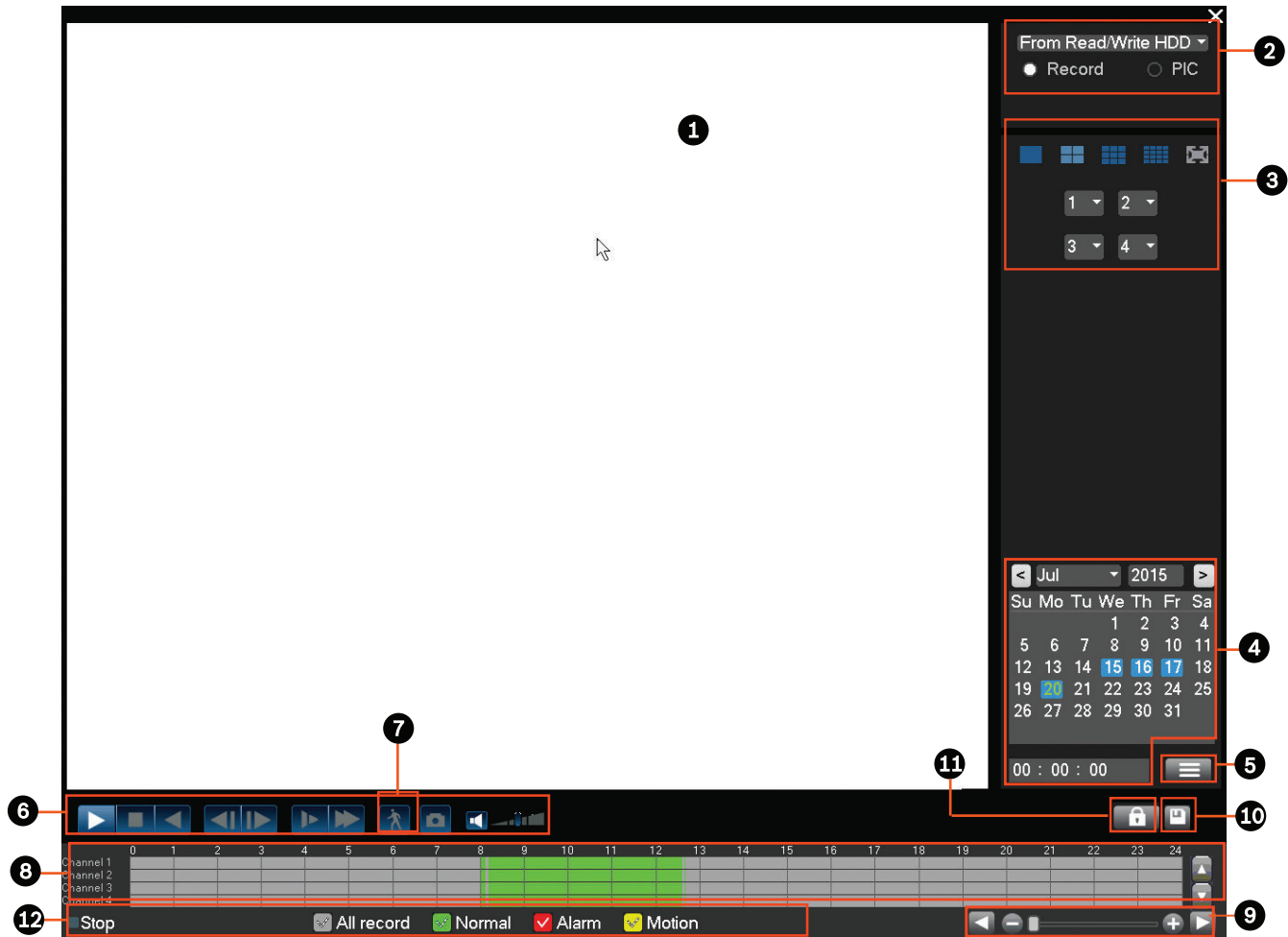
Figure 7.8: Search/Play screen
