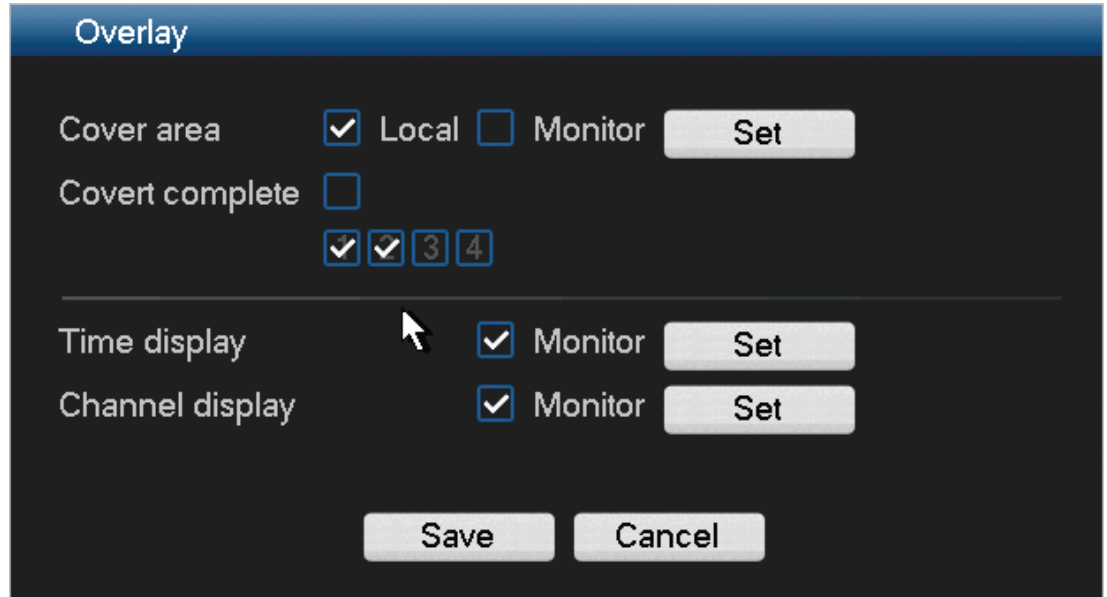
Figure 6.5: Encode overlay
