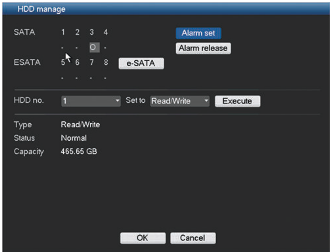
Figure 6.30: Hard disk
