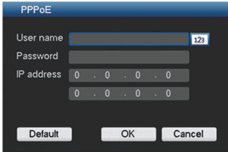
Figure 6.14: Network PPPoE
