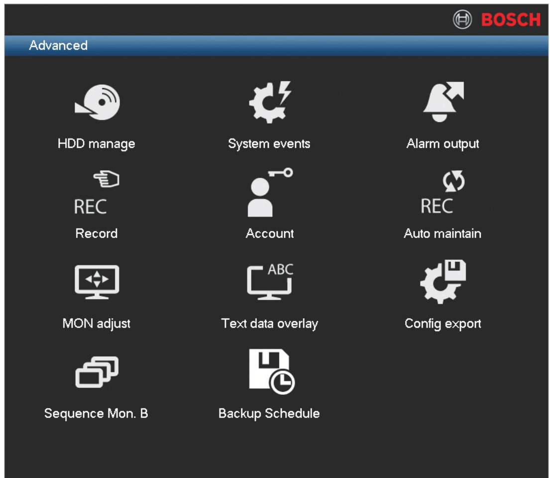
Figure 6.29: Advanced
