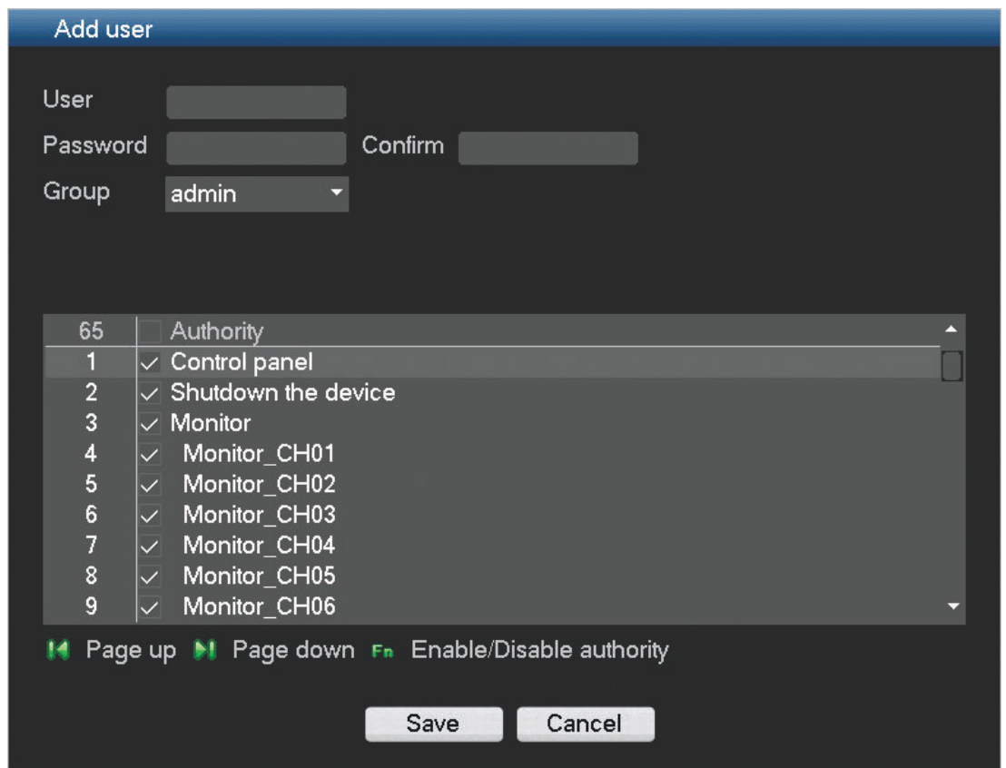
Figure 6.35: Add user
