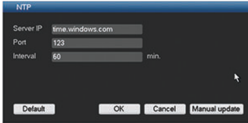
Figure 6.13: Network NTP
