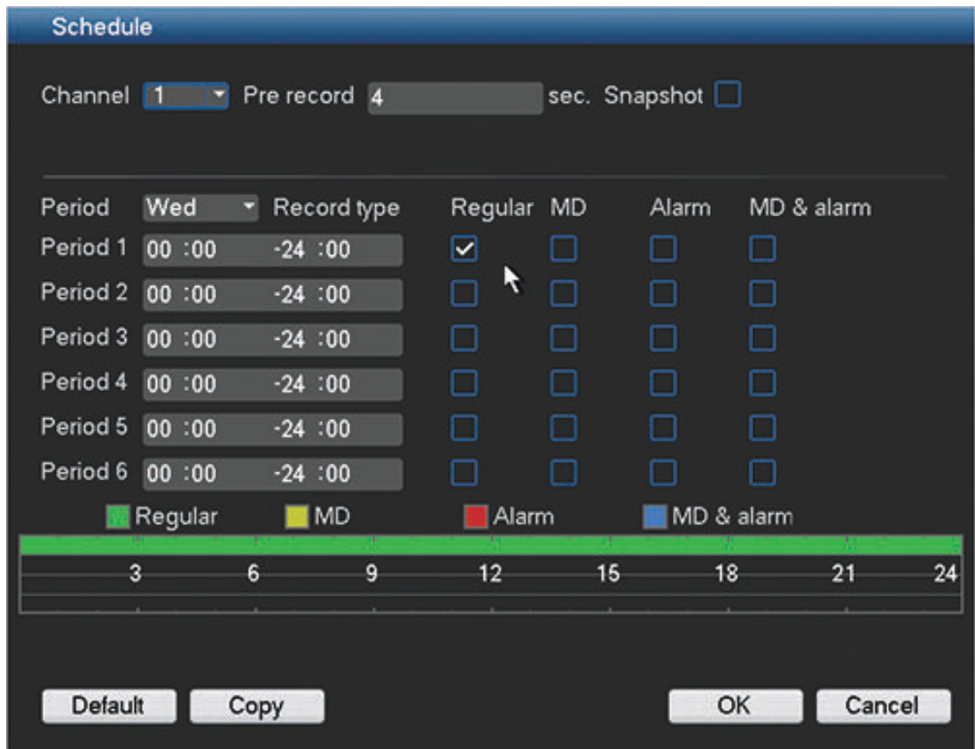
Figure 6.7: Schedule
