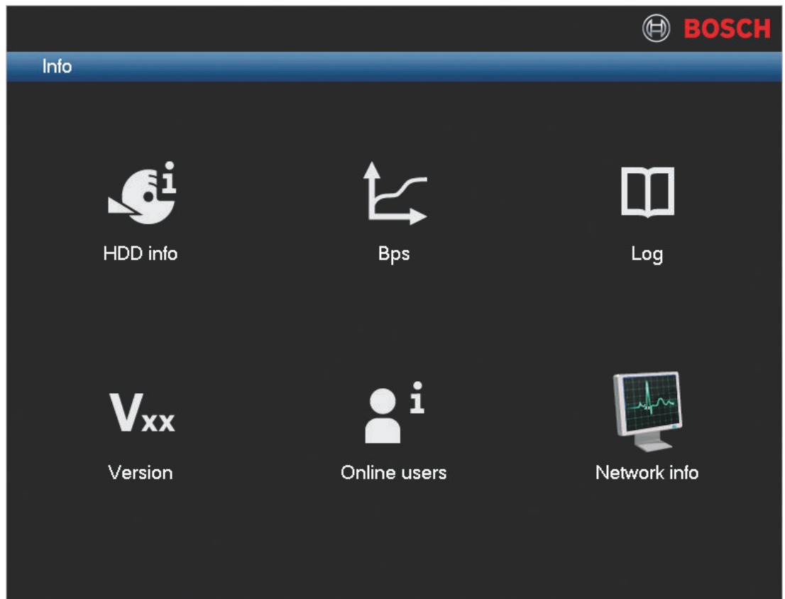
Figure 7.10: Info menu
