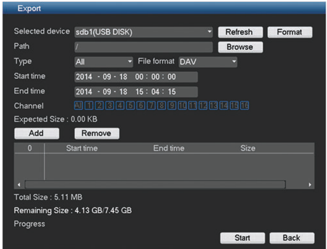
Figure 7.9: Export screen
