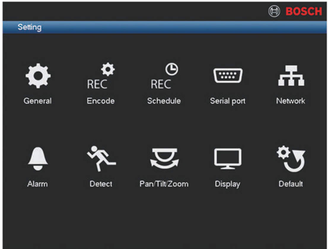
Figure 6.2: Settings
