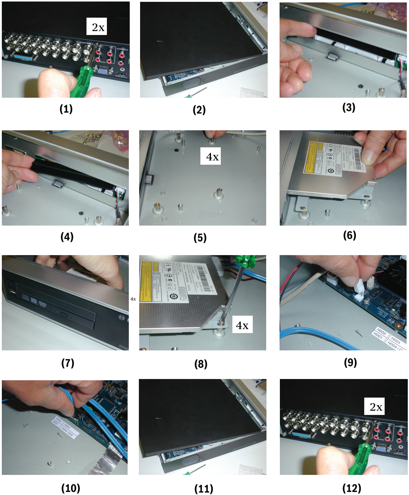
Figure 11.10: Install DVD in DIVAR AN 5000
