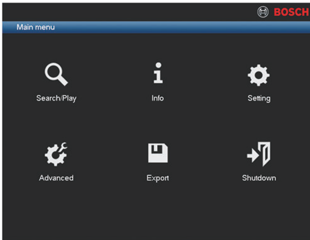
Figure 6.1: Main menu
