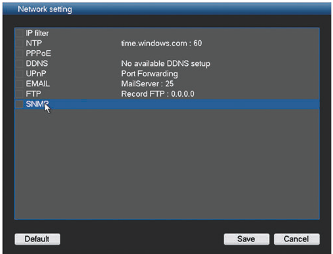
Figure 6.11: Network setting
