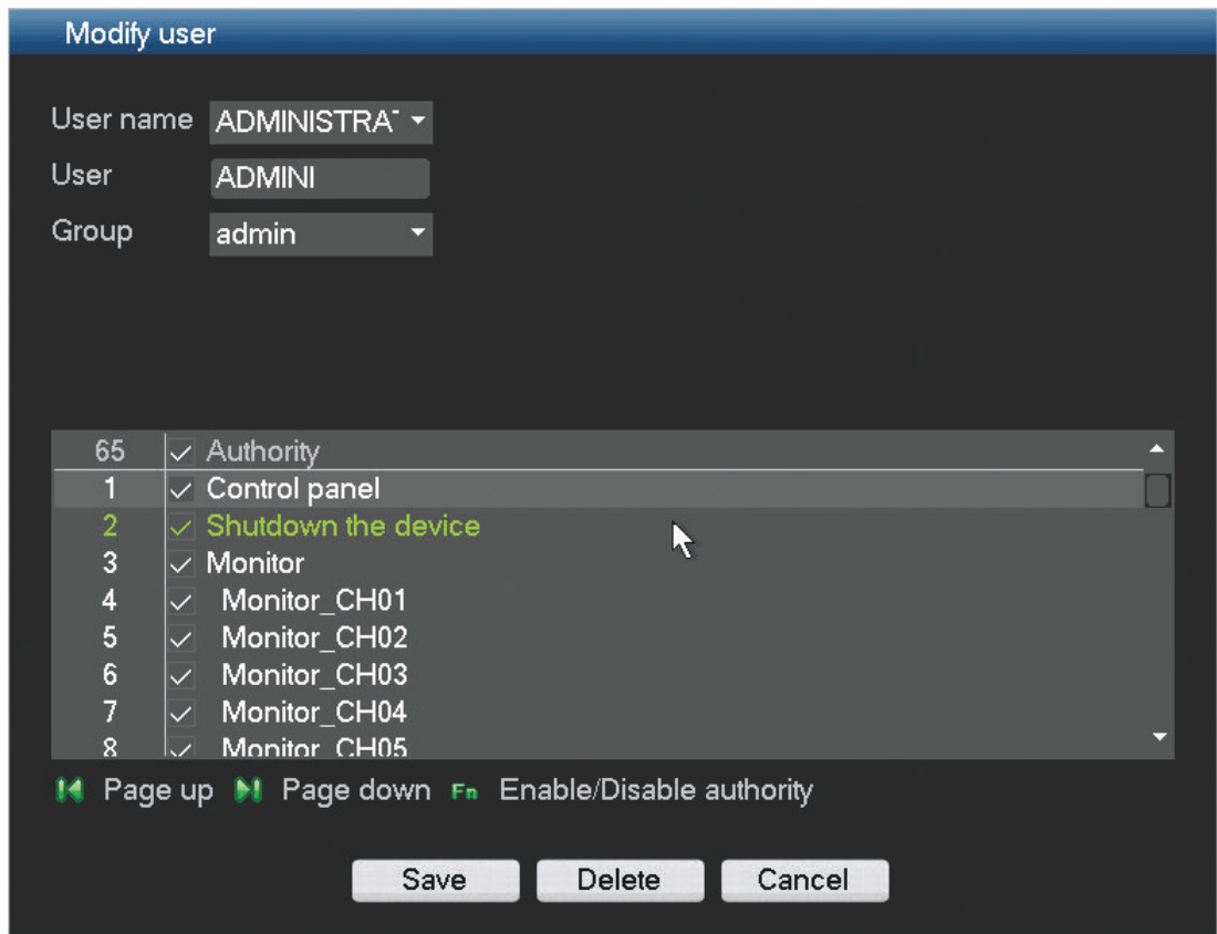
Figure 6.36: Modify user
