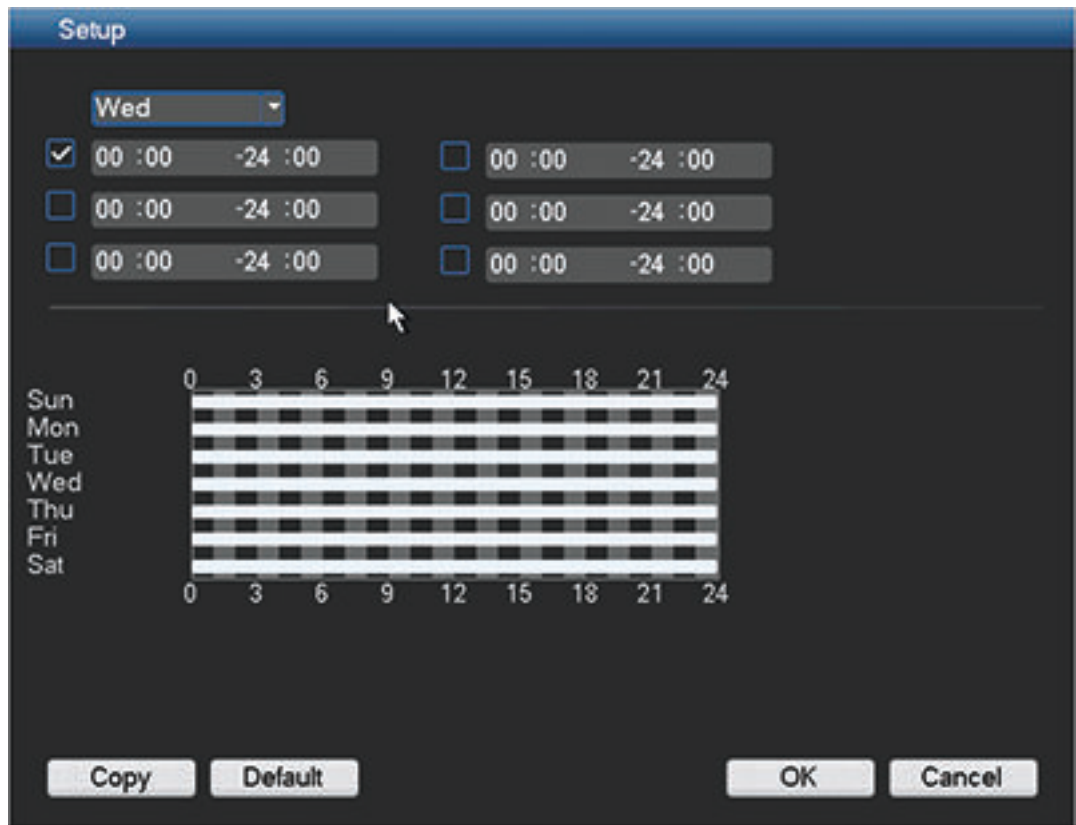
Figure 6.23: Period setup
