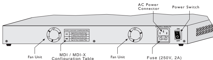
Figure 2 – KNS1600/R Rear Panel
