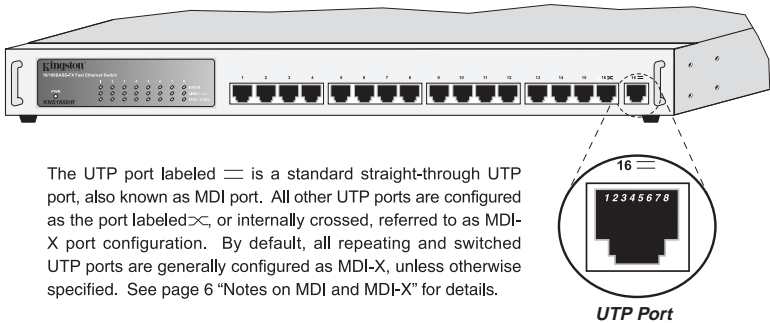
Fig. A-1 RJ-45 Connector Pin Numbers
