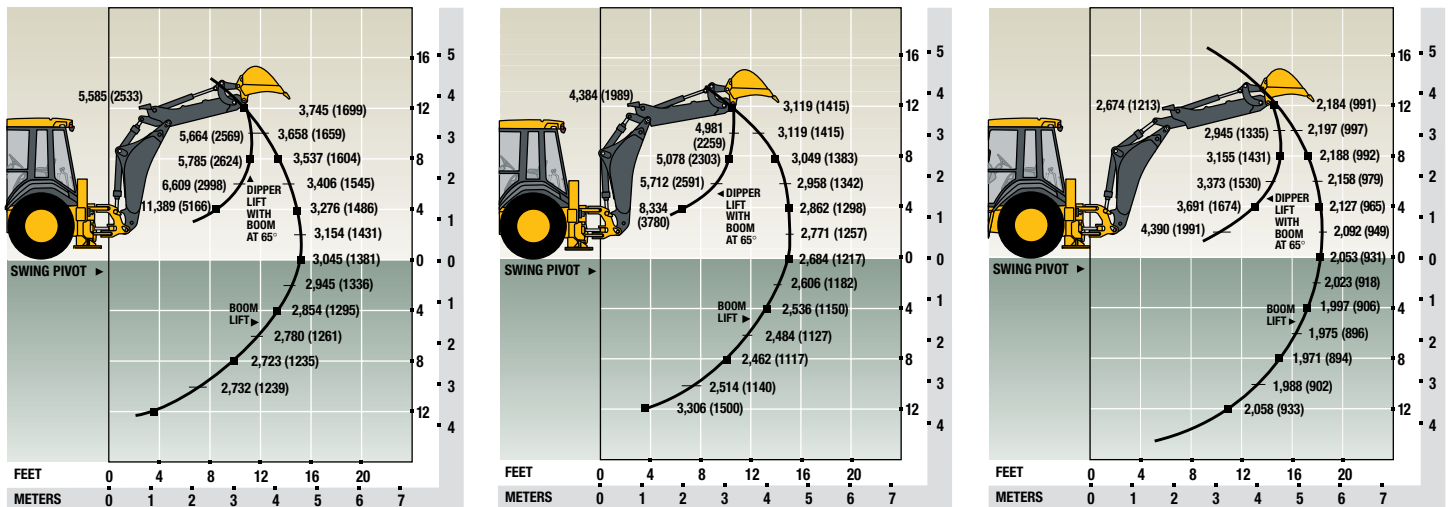
315SJ Backhoe with 3-ft. 6-in. (1.07 m) Extendable Dipperstick, Retracted
