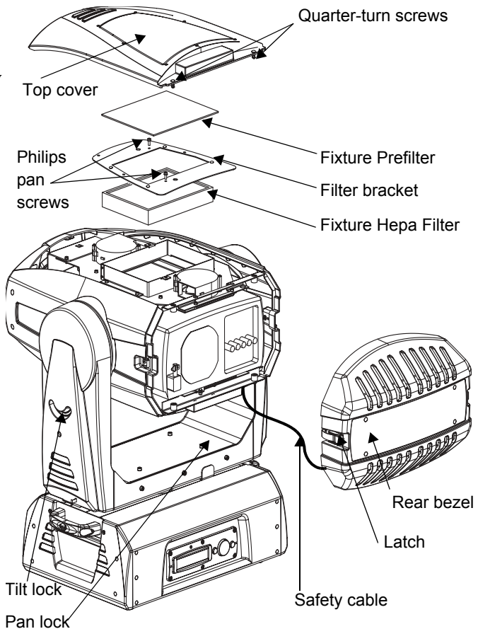
Figure 5-1 Replacing the Projector Filter
