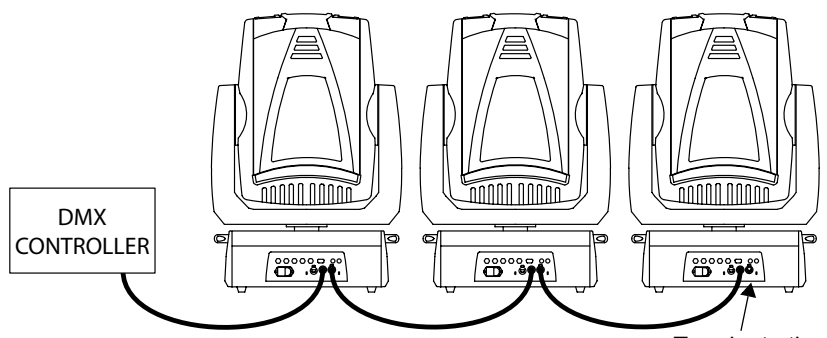
Figure 2-6 Linking DL.1 Fixtures
