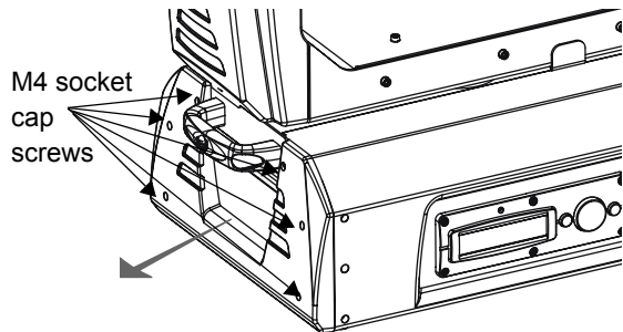
Figure 5-7 Accessing CPU and 3-phase boards.
