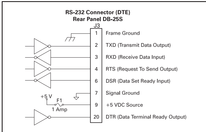
Figure 24. RS-232 Connections
