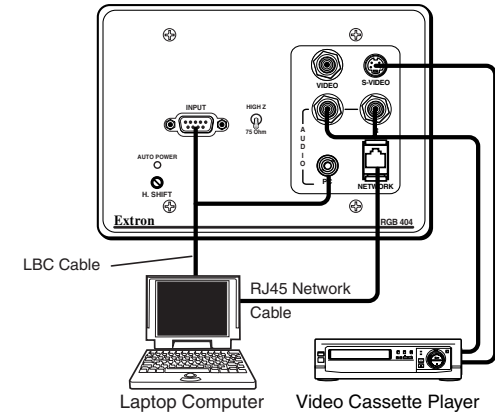
An RGB 404 application featuring a laptop and network and S-video pass-through connections
