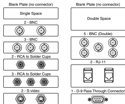
Architectural adapter plates
