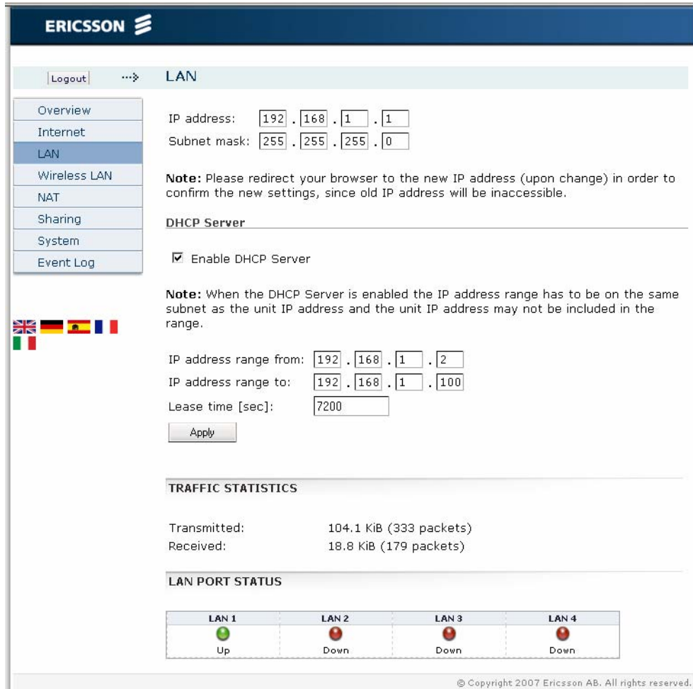
Figure 27 - LAN page
