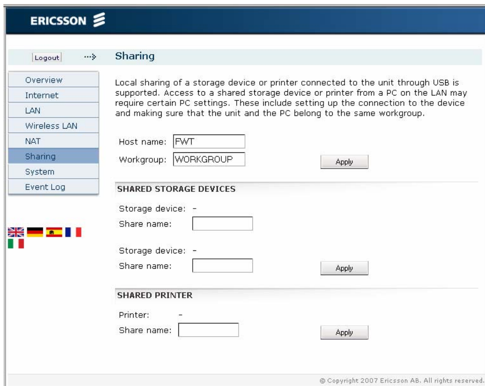
Figure 35 - Sharing page
