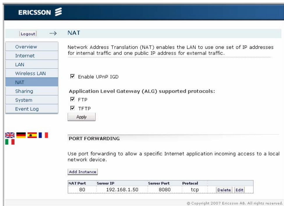
Figure 31 - NAT page
