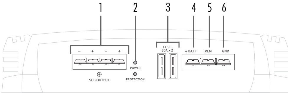
FIGURE 2—AMPLIFIER CONNECTIONS 600d REAR
