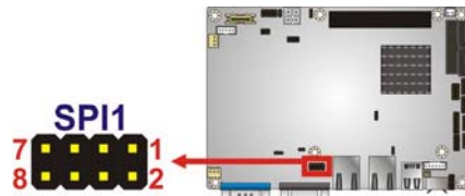
Figure 3-20: SPI Flash Connector
