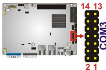
Figure 3-19: Serial Port Connector Location
