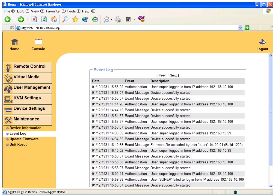
Figure 6-32. Event Log List
