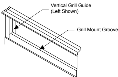
Location of Mounting Groove (RV Shown)
