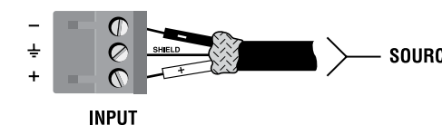
Figure 3.3 Balanced Input Connector Wiring
