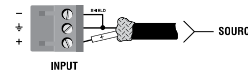
Figure 3.4 Unbalanced Input Connector Wiring
