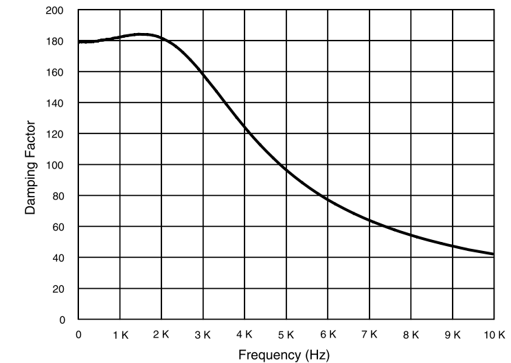
Figure 7.5 CTs 8200 Typical Damping Factor vs. Frequency
