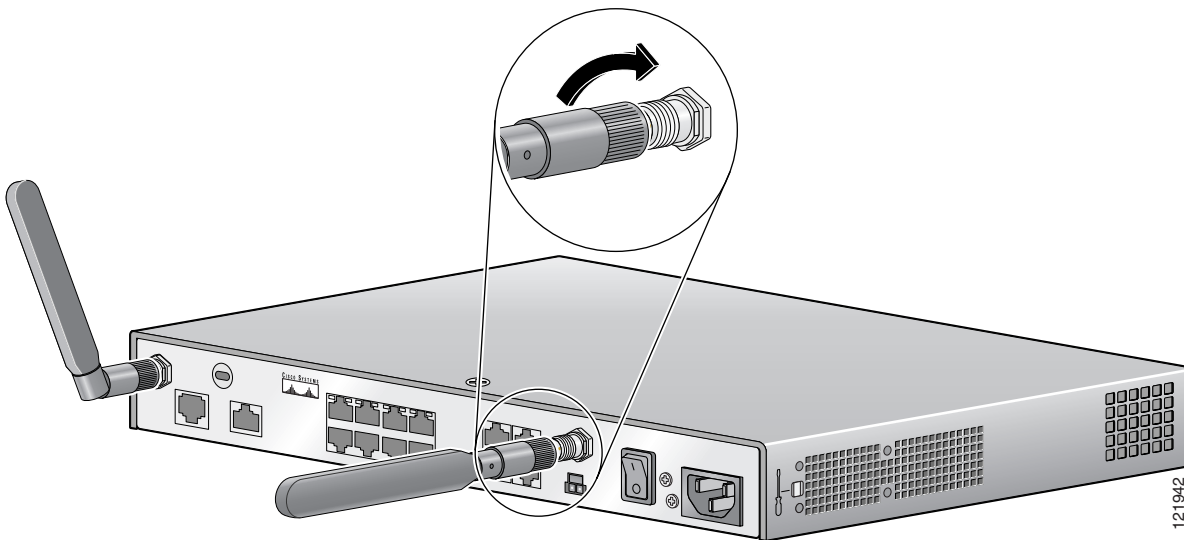
Figure 3 Connecting Antennas to the Router
