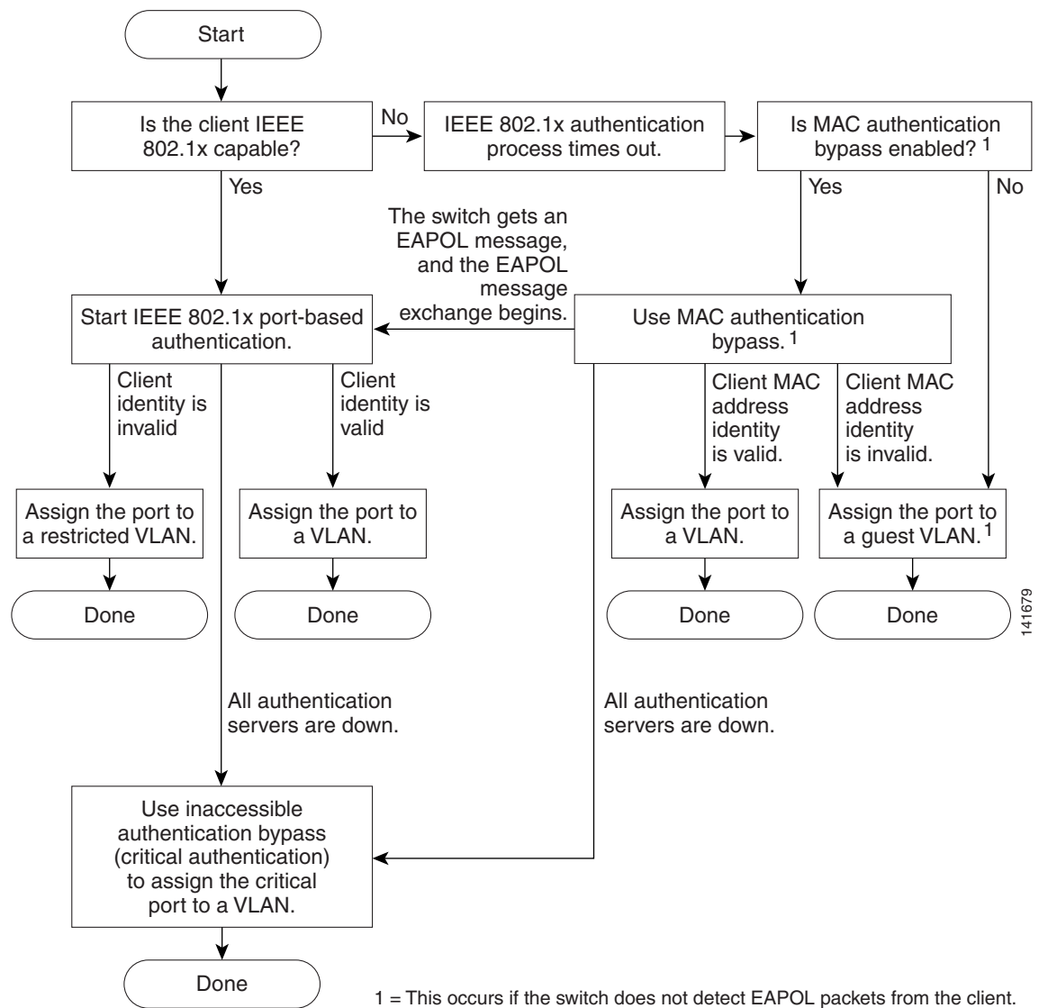
Figure 10-2 Authentication Flowchart
