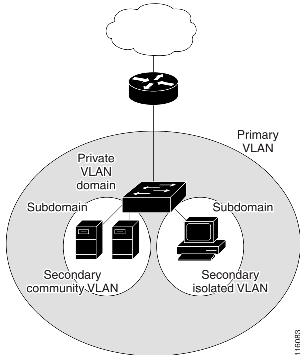
Figure 14-1 Private-VLAN Domain
