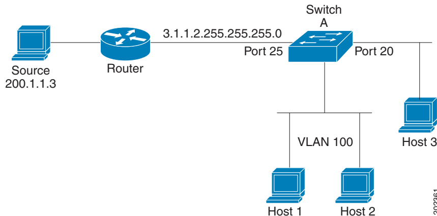
Figure 44-2 PIM Stub Router Configuration
