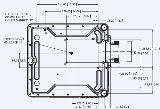
Underneath view
