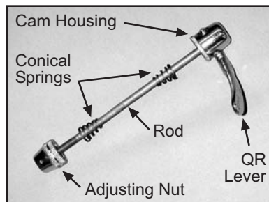
Fig. 2: Front QR anatomy shown properly assembled.
