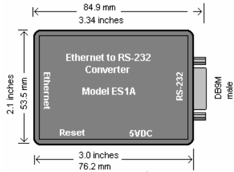
Figure 2. Top View of the ES1A Converter
