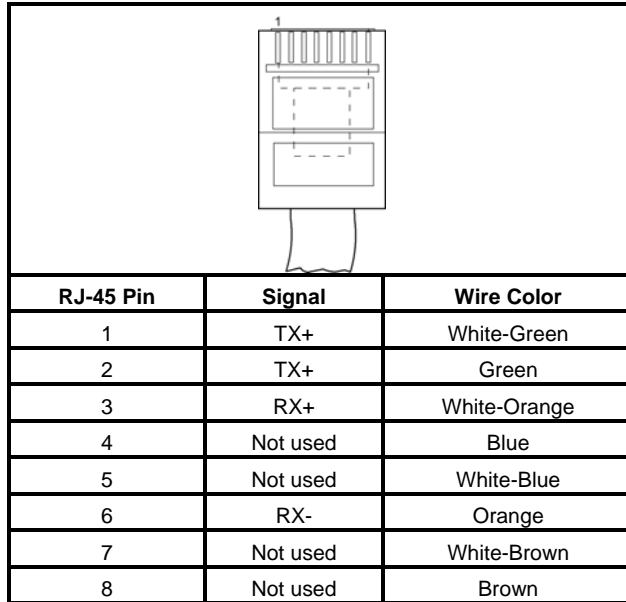
Figure 17. Pin-out for an Ethernet Cable
