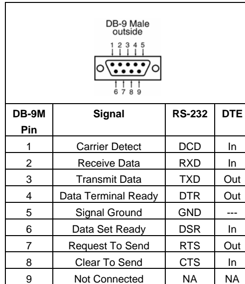
Figure 16. RS-232 Connections in a DB-9 Connector
