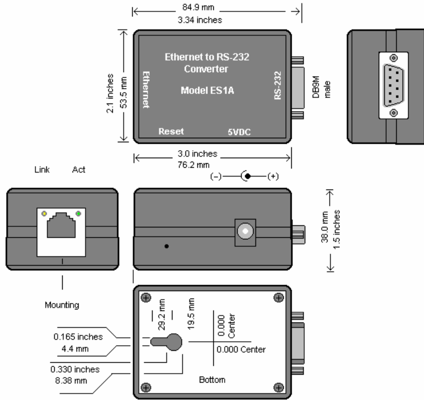
Figure 15. Dimensional Diagram of the ES1A
