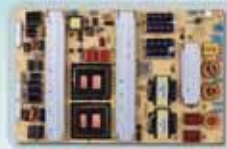
Ultra-thin LED TV power board • Input: 90-264V AC, 50/60Hz • Output: 24V DC/8A, 12V DC/3A, 5V DC/2.4A, 5V DC/0.5A • Max. power: 250W
