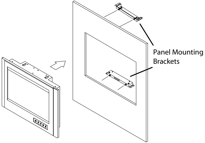
Figure 2.2: Panel Mounting (396 x 296 mm)
