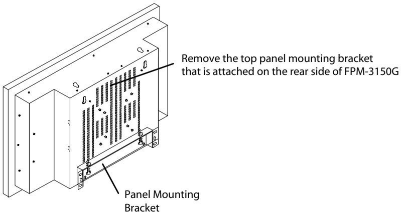
Figure 2.4: Desktop Stand for FPM-3150G
