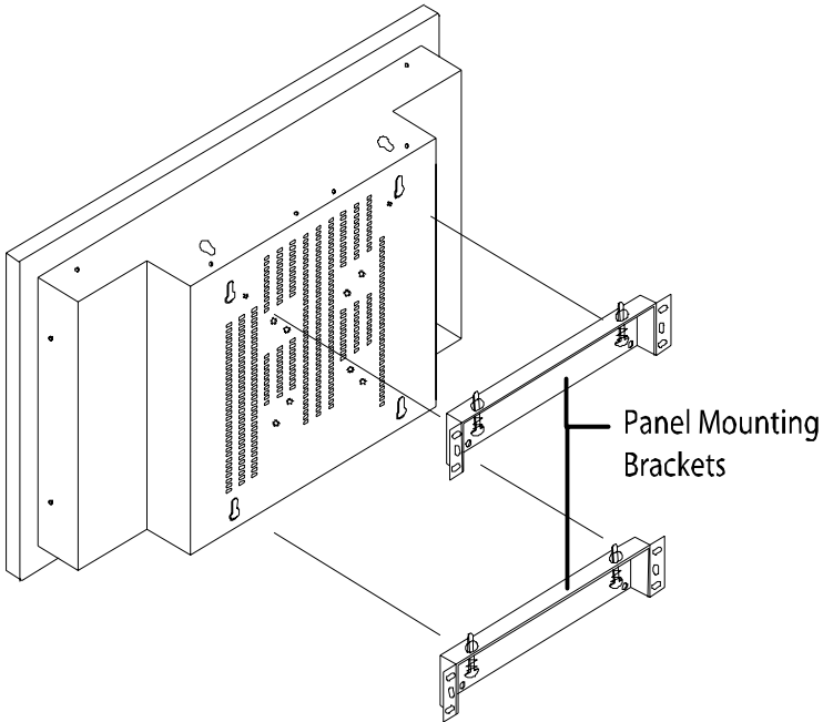
Figure 2.1: Wallmounting
