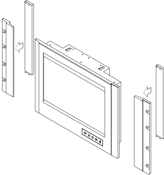
Figure 2.3: Rack Mounting Brackets
