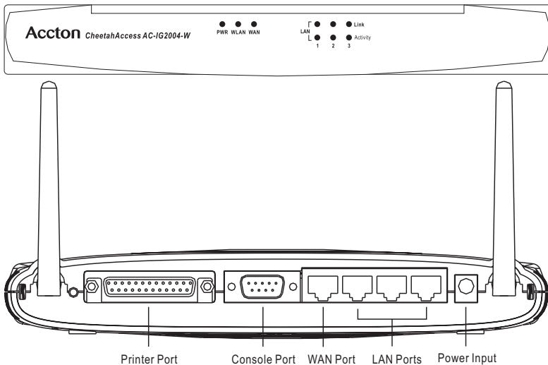
Figure 2-1. Front and Rear Panels
